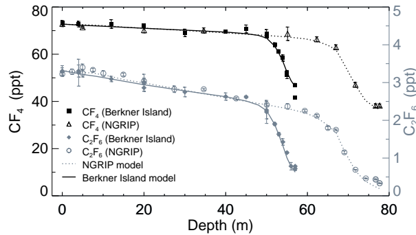
Figure 7. \text{CF}_4 and \text{C}_2\text{F}_6 at Berkner Island and North GRIP. Symbols show measurements from (Worton et al., 2007) Worton et al. (2007), that were not used in our inversions. Lines show modelled depth profiles created by convolving our inferred atmospheric mole fraction timeseries in the appropriate hemisphere with Green's functions from the LGGE-GIPSA firm model. \text{CF}_4 is shown in black (left axis) and \text{C}_2\text{F}_6 in grey (right axis).
