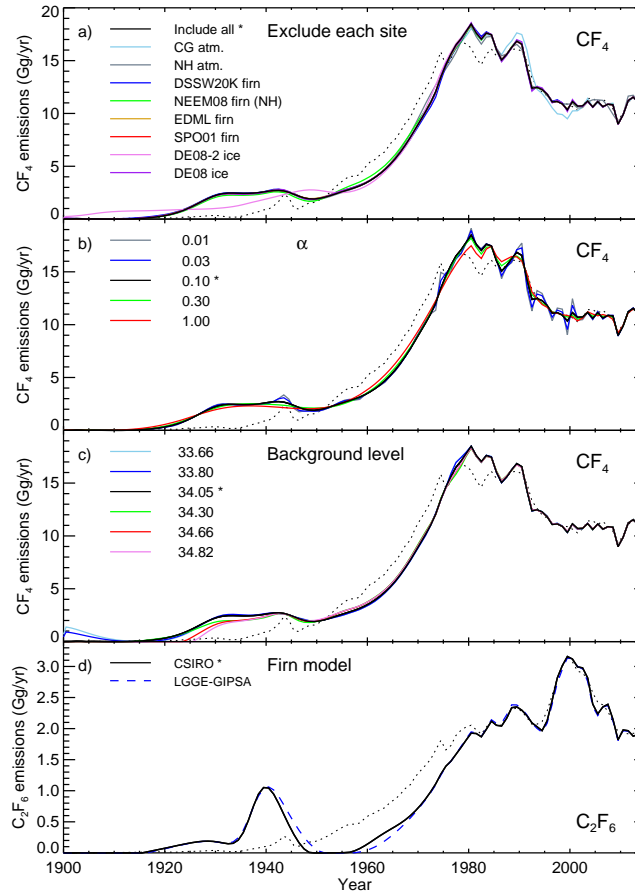
Figure 5. a) CF 4 emissions estimated by InvE2 with measurements from all sites (black), and with each site excluded one at a time. b) CF 4 emissions estimated using alternative values of the regularisation parameter \alpha . c) CF 4 emissions estimated using alternative values of the pre-industrial pre-anthropogenic background level. d) C 2 F 6 emissions inferred with the preferred Green's functions from the CSIRO (black solid line) and LGGE-GIPSA (blue dashed line) firm models. In all panels, our standard case is indicated in the legend by an asterisk, and the prior emissions are shown by the dotted lines.
