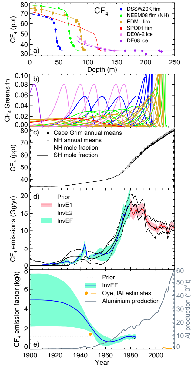
Figure 2. a) Depth profiles of CF 4 mole fraction in the firn and ice. Lines show model results corresponding to inferred emissions from InvE2; symbols are measurements with 1σ uncertainties. b) Green's functions from the CSIRO firn model (colors correspond to those in panel a)). c) Time history of mole fraction in the NH -northern hemisphere (NH, dashed line) and SH -southern hemisphere (SH, solid line) calculated with emissions inferred by InvE2. Symbols show annual values determined from atmospheric measurements in each hemisphere. d) Emissions inferred from the three inversions, with 95% confidence intervals. The dotted line shows the prior estimate based on a constant emission factor. e) Emission factor inferred by the InvEF inversion with 95% confidence intervals (blue), and constant prior (dotted). Emission factor estimated by Oye et al. (1999) for 1948 (orange circle) and recent estimates by the International Aluminium Institute (2014) (orange line, lower right corner). Primary aluminium production (U.S. Geological Survey, 2014; International Aluminium Institute, 2014) in 10 6 t (million metric tonnes) is shown with the grey line (right axis).
