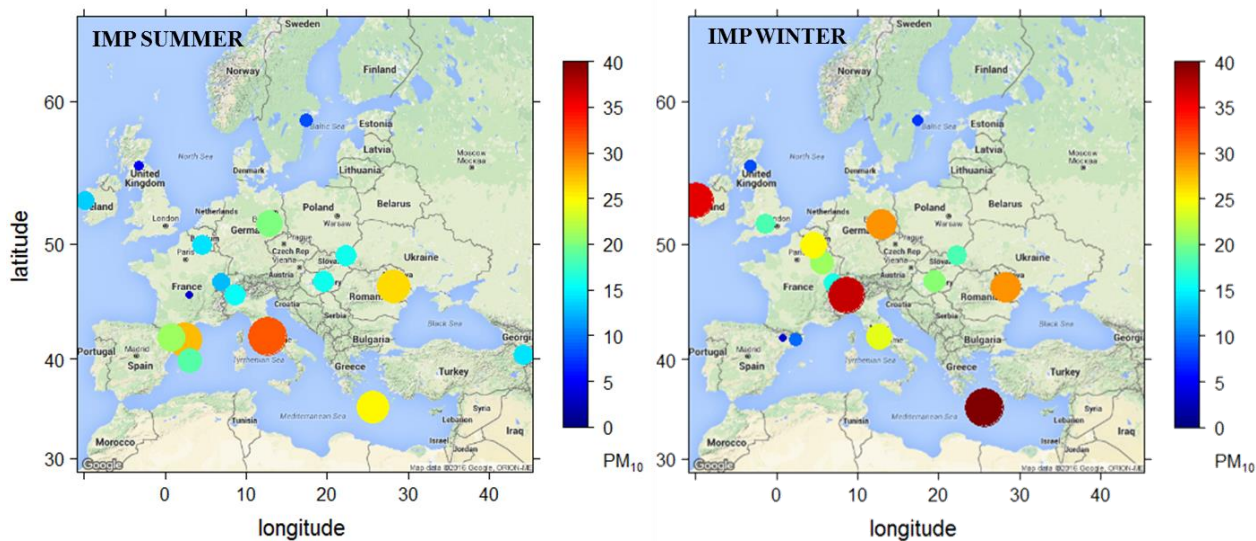
Figure 2: Mean PM_{10} concentrations ( \mu g m^{-3} ) recorded during the June/July 2012 and January/ February 2013 EMEP IMPs. The diameter of the circles is proportional to the concentrations.
