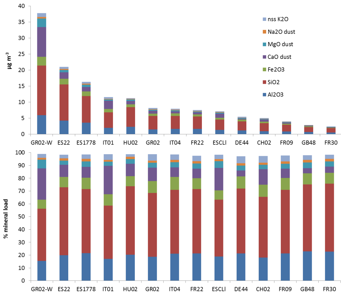
Figure 10: Average concentration of mineral dust components (absolute values – \mu\text{g m}^{-3} , top-) and the relative contribution of components (% , bottom) in mineral dust at selected sites when affected by African dust episodes. Results from both summer and winter (GR02-W) IMPs are included.
