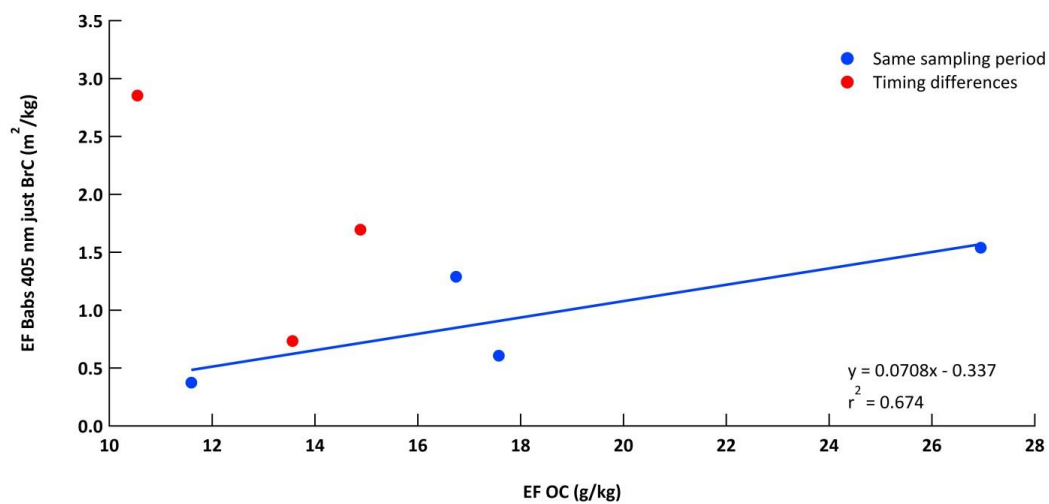
Figure 6. The estimated mass absorption coefficient of the bulk OC from the B_{\text{abs}} assigned to BrC versus simultaneously measured OC mass on filters. Only 4 plumes were sampled by both techniques over the exact same time period (blue symbols) and they were used in fit shown to estimate the MAC.
