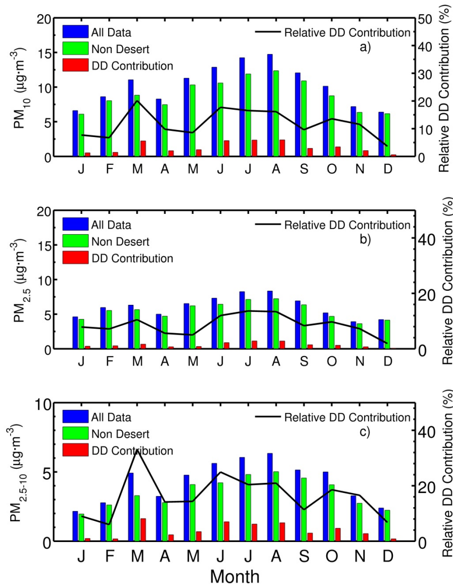
Figure 6: Annual cycle for DD contribution to the total monthly PM 10 (a), PM 2.5 (b), and PM 2.5-10 (c) means in absolute (red bar) and relative values (black line). Blue bars represent the annual cycle of total PM 10 (a), PM 2.5 (b), and PM 2.5-10 (c) and green bars the corresponding values without including the days of desert dust.
