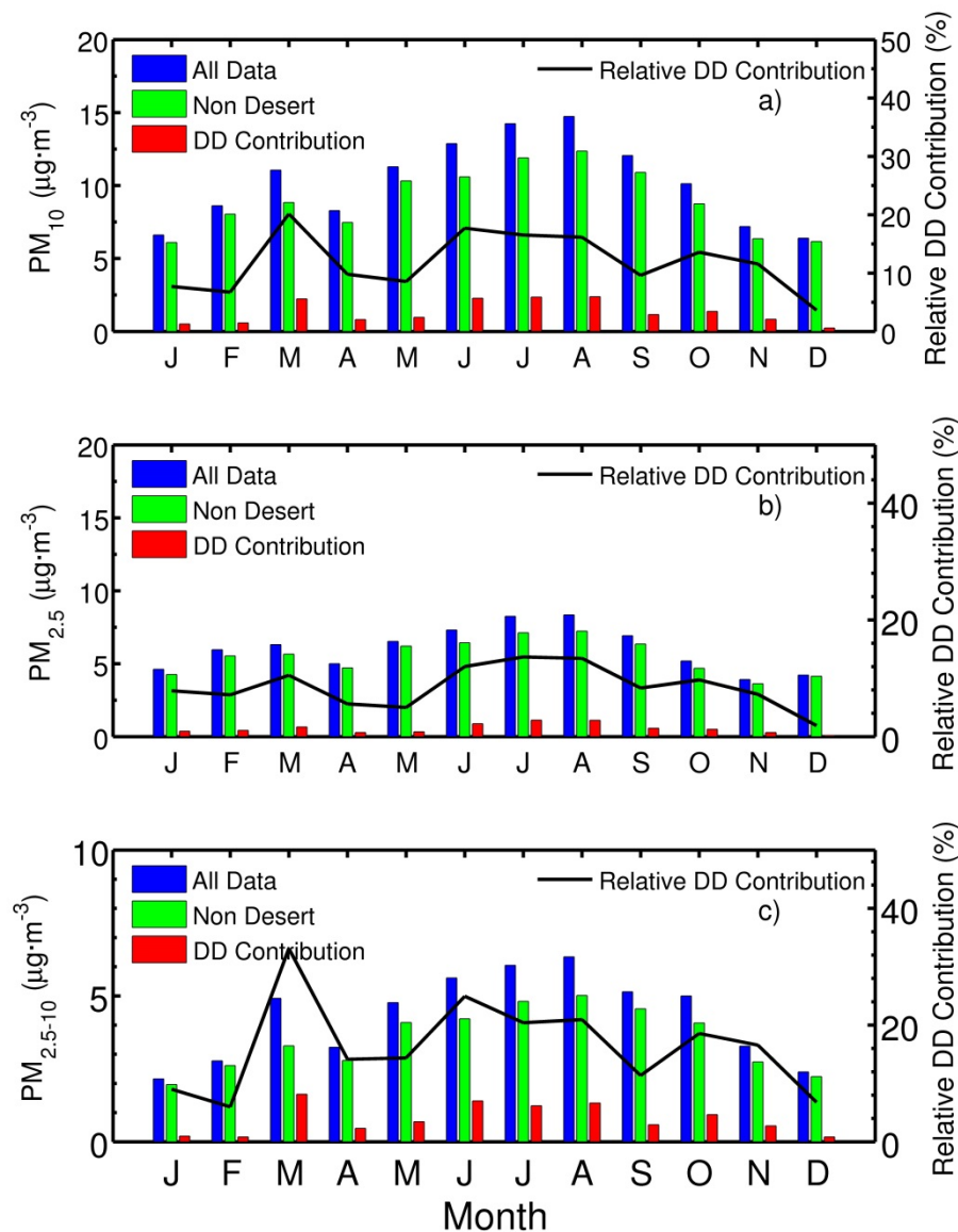
5 Figure 6: Annual cycle for DD contribution to the total monthly \text{PM}_{10} (a), \text{PM}_{2.5} (b), and \text{PM}_{2.5-10} (c) means in absolute (red bar) and relative values (black line) in 2003-2014. Blue bars represent the annual cycle of total \text{PM}_{10} (a), \text{PM}_{2.5} (b), and \text{PM}_{2.5-10} (c) and green bars the corresponding values without including the days of desert dust.
