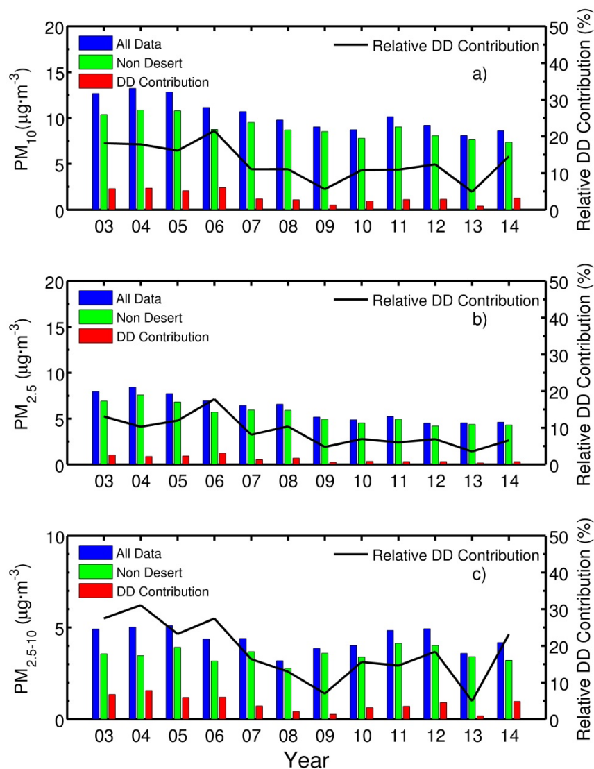
Figure 7: Inter-annual variability of DD contribution to the total yearly PM_{10} (a), PM_{2.5} (b), and PM_{2.5-10} (c) in absolute (red bar) and relative values (black line). Blue bars represent the mean year PM_{10} (a), PM_{2.5} (b), and PM_{2.5-10} (c) value and green bars the corresponding values without including the days of desert dust.
