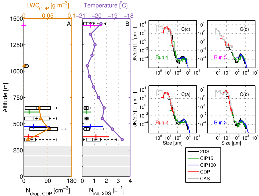
Figure 6. Microphysics summary of averaged observations over the sea ice. A: CDP droplet number concentration (boxes, black) with derived liquid-water content overlaid (orange). B: 2DS ice crystal number concentration (boxes, black) with mean temperature measured overlaid (purple). Only CDP and 2DS data >0.5 \text{ cm}^{-3} and >0.05 \text{ L}^{-1} respectively have been included. Box edges represent the 25 th and 75 th percentiles, and the median and mean values are denoted by | and + respectively. Altitudes not sampled are blocked out ( \leq 300\text{m} ). A and B: number concentrations from each SLR are shown in colour at each corresponding altitude (run 2: red, run 3: blue, run 4: green, run 5: magenta). Arithmetic means are indicated ( \bar{\phantom{x}} ) with each horizontal bar extending to \pm 1\sigma . C(a-d): Number size distributions ( dN/dD ) from each SLR over the sea ice (runs 2-5 respectively). Legend refers to panel C only.
