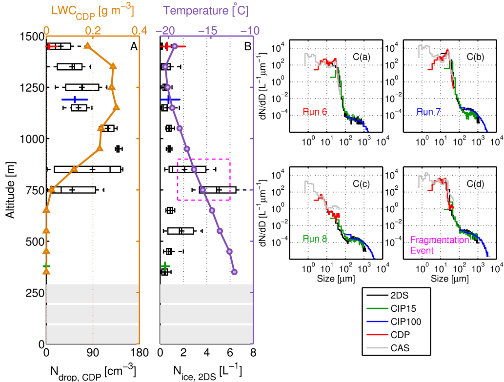
Figure 9. Microphysics summary of averaged observations over the ocean. Data are displayed similarly to Fig. 6. In panels A and B , data from each SLR are again shown in colour at each corresponding altitude (run 6: red, run 7: blue, run 8: green) as before. C(a-d) : Number size distributions ( dN/dD ) from each SLR over the ocean (runs 6-8). Legend refers to panel C only. High ice number concentrations at cloud base are labelled as a fragmentation event (see Sects. 4.1.2 and 5.3).
