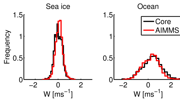
Figure 17. Probability density function (PDF) of updraught velocity from the core turbulence (black) and AIMMS (red) probes. Data from runs 2, 3 and 4 are used for the sea ice, and data from runs 6 and 7 for the ocean. Data from each SLR are normalised such that the mean value is zero.
