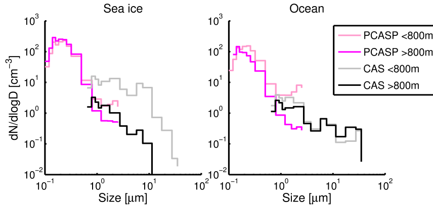
Figure 14. PCASP and CAS-DPOL particle size distributions over sea ice and ocean. Data are split into lower and higher than 800 m to reflect altitude influences. Only out of cloud (CDP LWC \leq 0.01 \text{ g m}^{-3} ) data are included.
