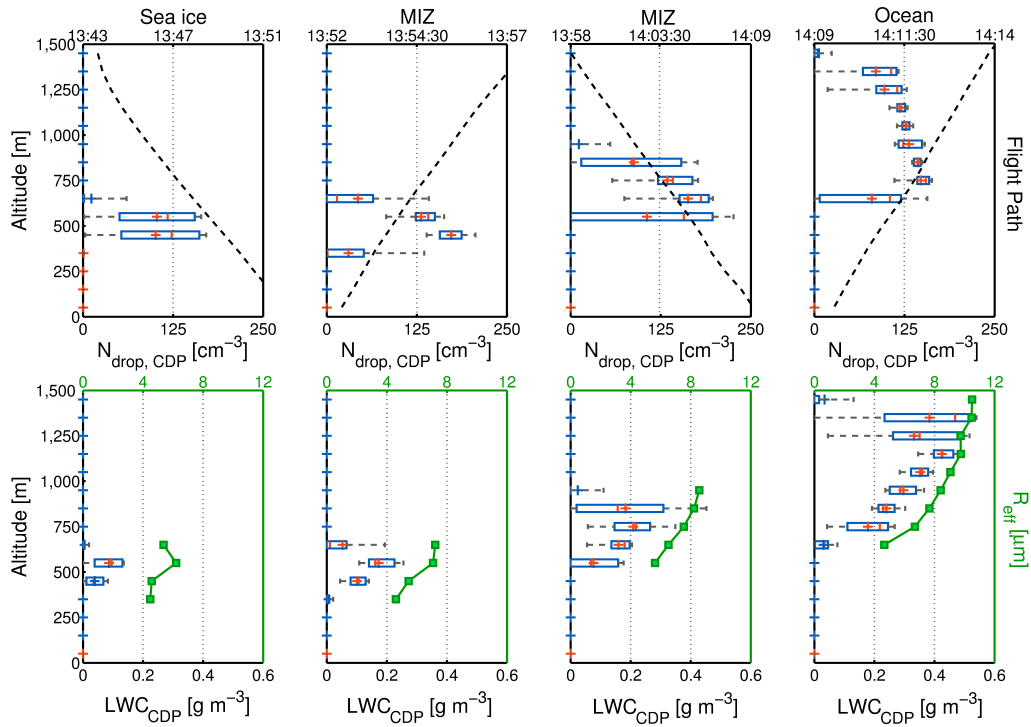
Figure 12. CDP data from the sawtooth profiles. Cloud droplet number concentration ( \text{cm}^{-3} , top row ) and derived LWC ( \text{g m}^{-3} , bottom row ) are shown. Box edges again indicate the 25 % and 75 % thresholds of the data, mean values are shown as a red cross and outliers extend to the 10 % and 90 % thresholds of the data. The altitude of the aircraft is indicated (black, dashed) in the top row and mean droplet effective radius – in \mu\text{m} , derived from CDP measurements – is shown (green) in the bottom row. Columns indicate the different profiles, transitioning from sea ice to ocean from left to right.
