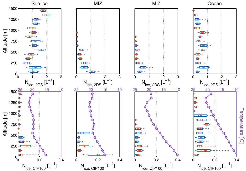
Figure 13. Ice number concentrations ( L^{-1} ) from the 2DS and CIP100 from the sawtooth profiles over the transition region. Data are displayed similarly to Fig.12. Temperature is overlaid (purple) in the bottom row.
