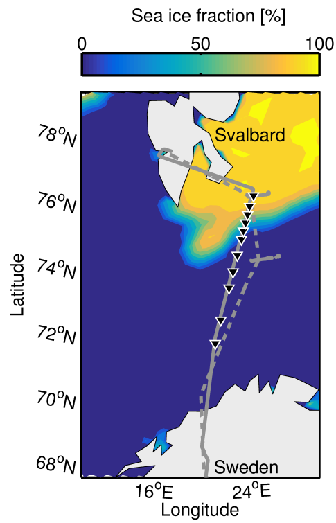
Figure 1. Flight track for B762 on 23 March 2013 over sea ice concentration fraction (shading). Section 1 of the flight (grey, solid) was conducted at a high altitude, where 11 dropsondes (black triangles) were released. Section 2 of the flight (grey, dashed) conducted straight, level runs over the sea ice and open water, with a sawtooth profile over the transition region.
