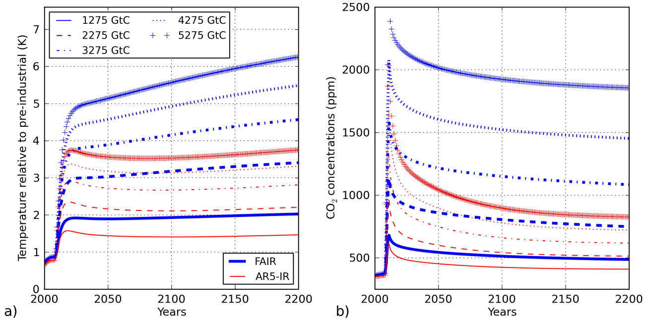
Figure 5. Dependency of temperature response on pulse size. Panel a) shows the global mean surface temperature response to the pulse experiments of Herrington and Zickfeld (2014). Responses are shown for the FAIR (blue) and AR5-IR (red) models. Panel b) shows the corresponding concentration response.
