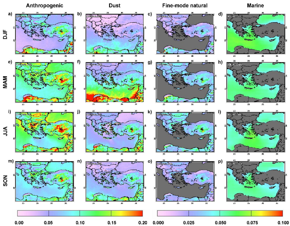
1 2 3 Figure 11. Seasonal (a, e, i, m) anthropogenic aerosol ( \tau_a ), (b, f, j, n) dust ( \tau_d ), (c, g, k, o) fine 4 mode natural aerosol ( \tau_n ) and (d, h, i, p) marine aerosol ( \tau_m ) patterns over the Eastern 5 Mediterranean based on MODIS Terra observations during the period 3/2000-12/2012 6 (3/2000-12/2007 for regions of North Africa covered by DB data only).
