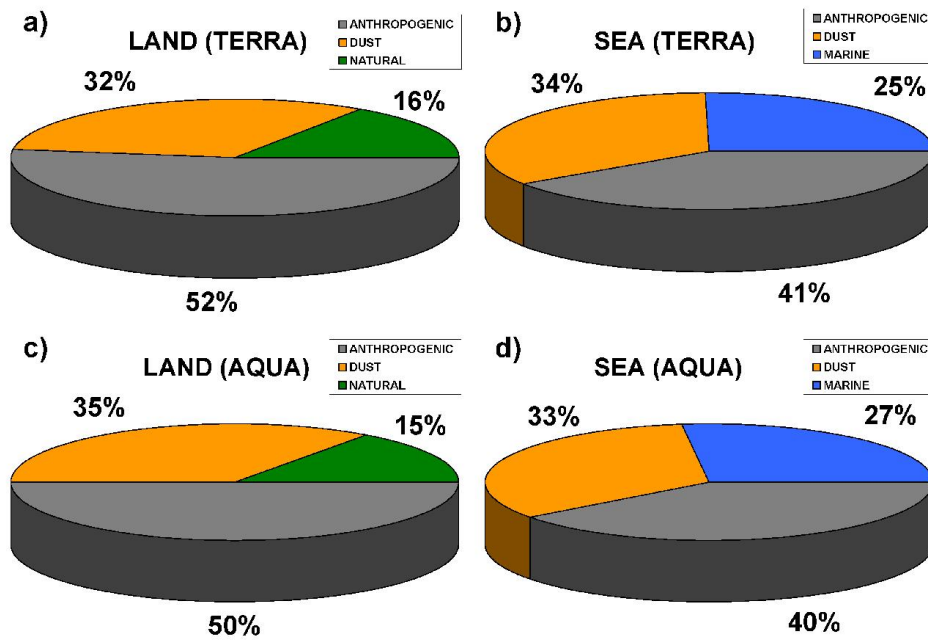
1 2 3 Figure 7. Relative contribution of anthropogenic aerosols, dust and fine mode natural 4 aerosols to the total AOD 550 over the land covered part of Eastern Mediterranean based on 5 MODIS Terra (a) and MODIS Aqua (c) observations and relative contribution of 6 anthropogenic aerosols, dust and marine aerosols to the total AOD 550 over the oceanic part of 7 Eastern Mediterranean based on MODIS Terra (b) and MODIS Aqua (d) observations.
