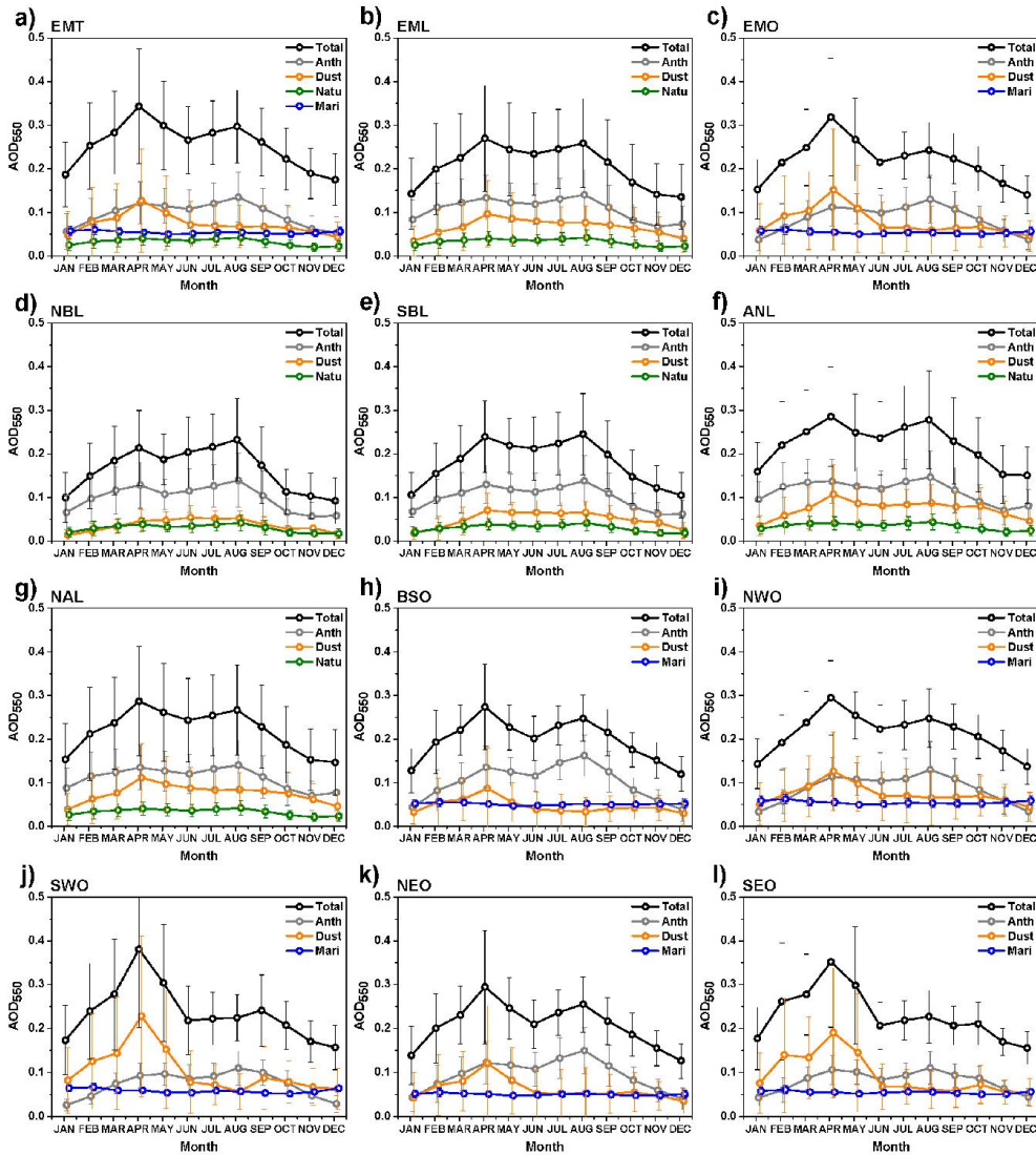
1 2 3 Figure 12. Seasonal variability of anthropogenic aerosols ( \tau_a ), dust ( \tau_d ), fine mode natural 4 aerosols ( \tau_n ) and marine aerosols ( \tau_m ) over Eastern Mediterranean (EMT), over the land 5 covered part (EML), over the oceanic part (EMO) and over the 9 sub-regions of the Eastern 6 Mediterranean appearing in Fig. 1 based on MODIS Terra observations. The error bars 7 represent the \pm 1\sigma values calculated from monthly gridded data.
