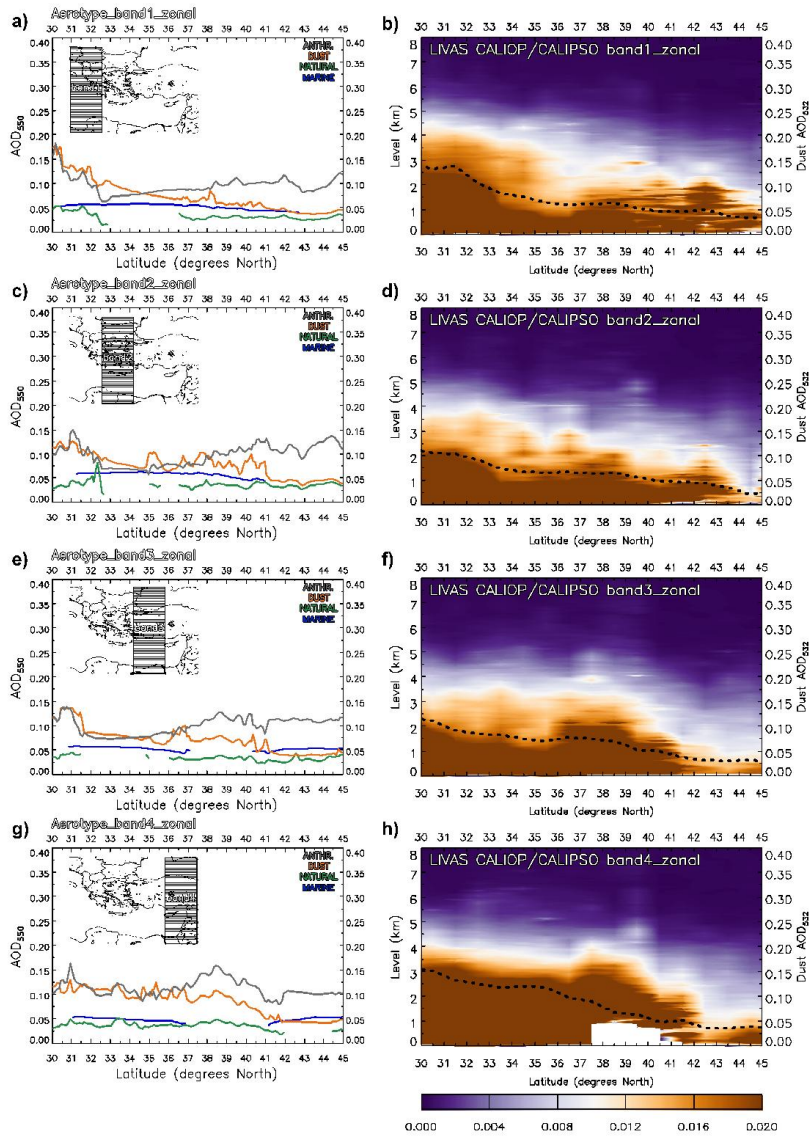
1 2 3 Figure 9. Left column: Latitudinal variability of anthropogenic aerosols ( \tau_a ), dust ( \tau_d ), fine 4 mode natural aerosols ( \tau_n ) and marine aerosols ( \tau_m ) for four 5-degree longitudinal bands (see 5 embedded maps) covering Eastern Mediterranean based on MODIS Terra observations. Right 6 column: Latitudinal variability of dust extinction coefficients at 532 nm in km -1 (colorscale 7 corresponds to the extinction coefficients and left y-axis to the atmospheric levels) and dust 8 aerosol optical depth at 532 nm (dotted line corresponding to the right-y-axis) for the same 9 four bands from LIVAS CALIOP/CALIPSO observations.
