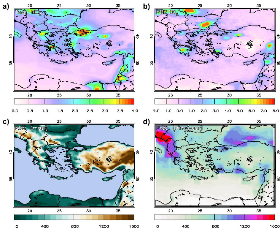
12 13 14 Figure 5. (a) Tropospheric NO 2 levels and (b) Planetary boundary layer SO 2 levels (in 10 15 15 molecules/cm 2 ) over the Eastern Mediterranean as seen from OMI/AURA (2005-2012), (c) 16 Topography (GTOPO elevation data in meters above sea level) and (d) Annual precipitation
