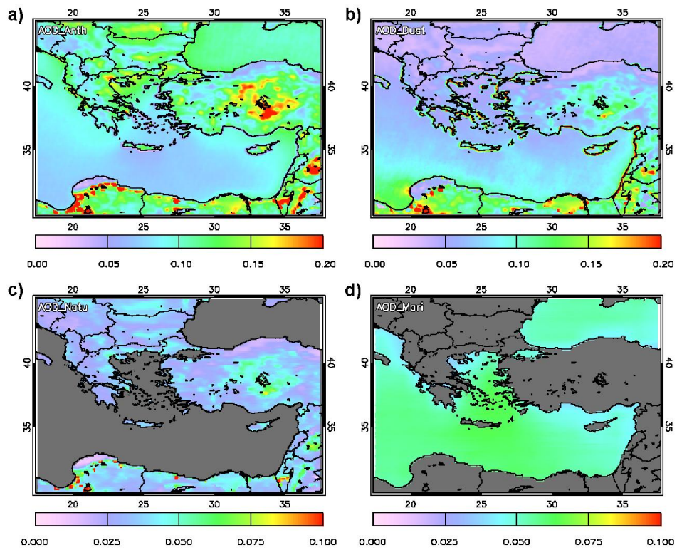
1 2 3 Figure 8. (a) Anthropogenic aerosol ( \tau_a ), (b) dust ( \tau_d ), (c) fine mode natural aerosol ( \tau_n ) and 4 (d) marine aerosol ( \tau_m ) patterns over the Eastern Mediterranean based on MODIS Terra 5 observations during the period 3/2000-12/2012 (3/2000-12/2007 for regions of North Africa 6 covered by DB data only).
