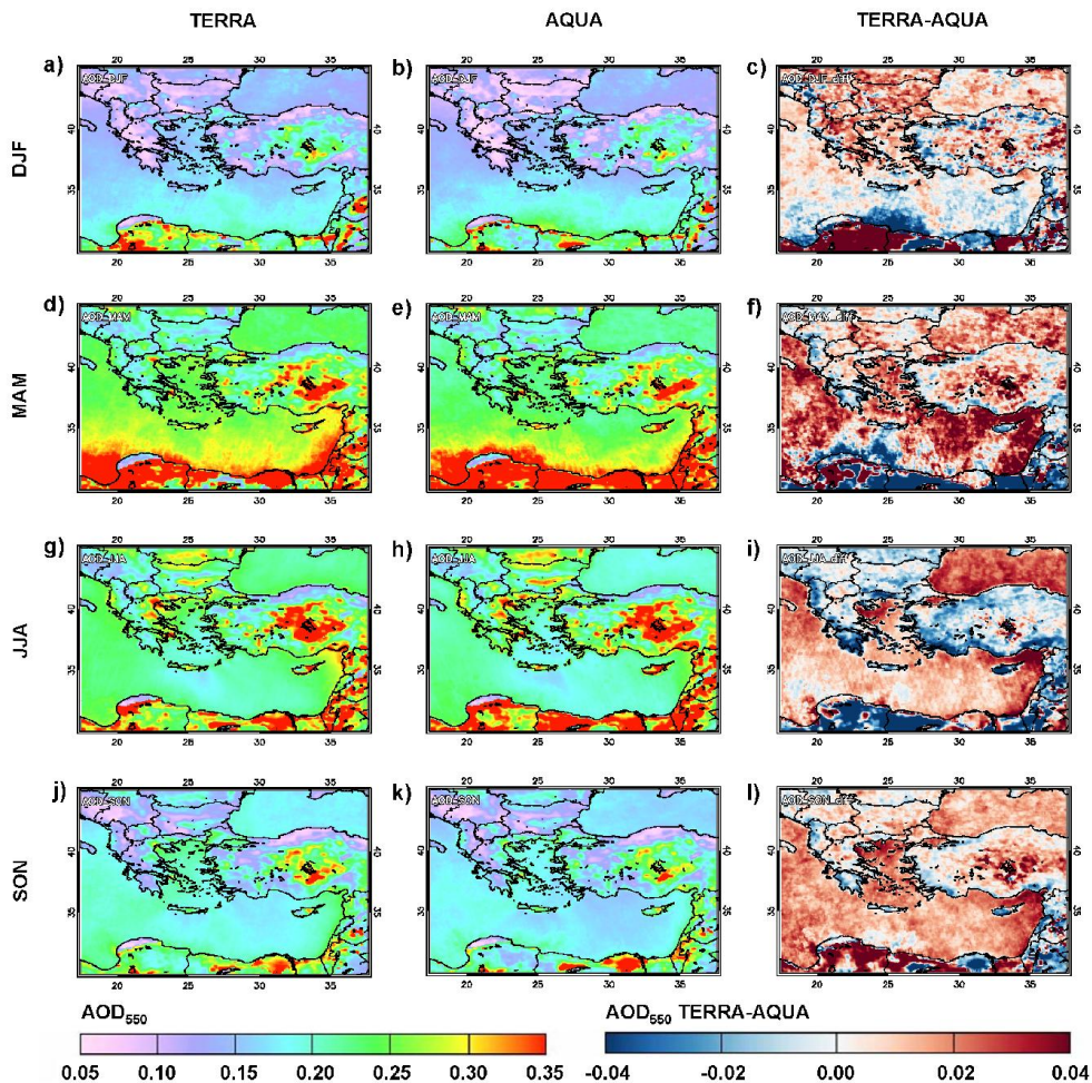
3 4 5 Figure 6. Seasonal AOD 550 patterns over the Eastern Mediterranean as seen by MODIS Terra 6 (left column) during the period 3/2000-12/2012 (3/2000-12/2007 for regions of North Africa 7 covered by DB data only) and MODIS Aqua (middle column) during the period 7/2002- 8 12/2012. The differences between MODIS Terra and Aqua AOD 550 on a seasonal basis appear 9 on the right column.
