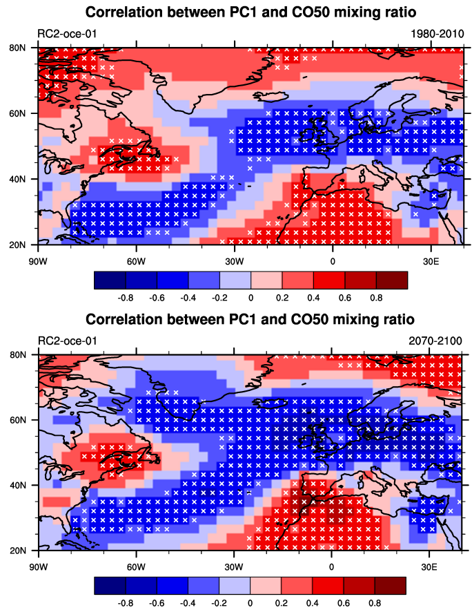
Figure 1: Correlation between the winter seasonal CO_{50} mixing ratio anomalies at the surface level and the PC1 of SLP computed with the coupled simulation data for the period (A) ( top ) and (B) ( bottom ). Points marked with a white cross indicate local significance at the 95%.
