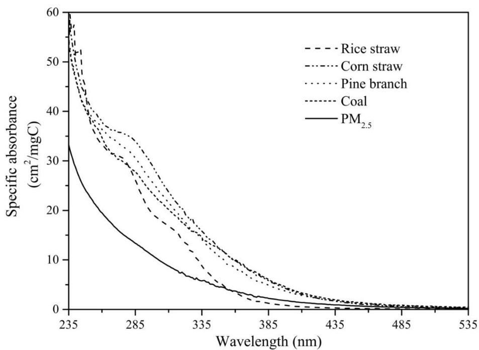
Figure 1. The normalized UV-vis spectra with TOC (units: \text{cm}^2/\text{mgC} ) of HULIS in smoke \text{PM}_{2.5} from combustion of rice straw, corn straw, pine branch and coal, and in ambient \text{PM}_{2.5} .
