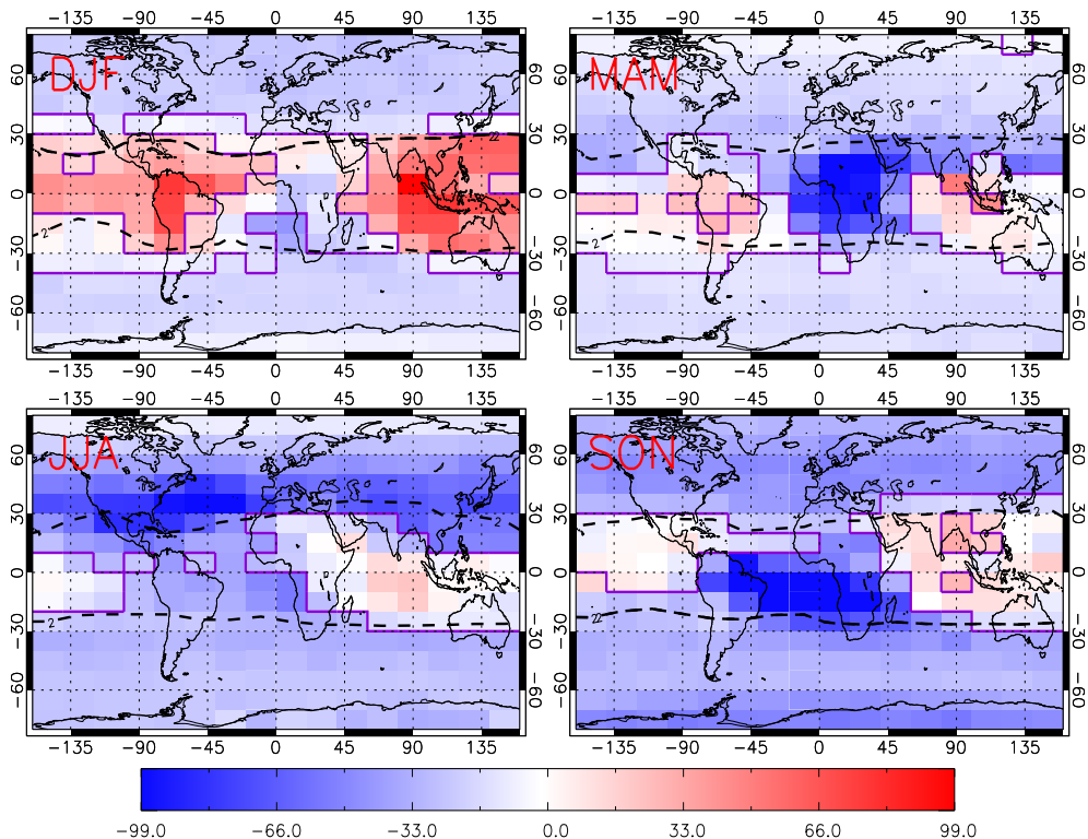
Fig. 12. Difference in PAN (pptv) between the TOMCAT model (with IMK AKs applied) and observed IMK MIPAS PAN at 150 hPa for 2007-2008 in DJF, MAM, JJA and SON. Purple polygonned areas show regions of significant differences, where the |\text{TOMCAT} - \text{observations}| > \text{observational error} .
