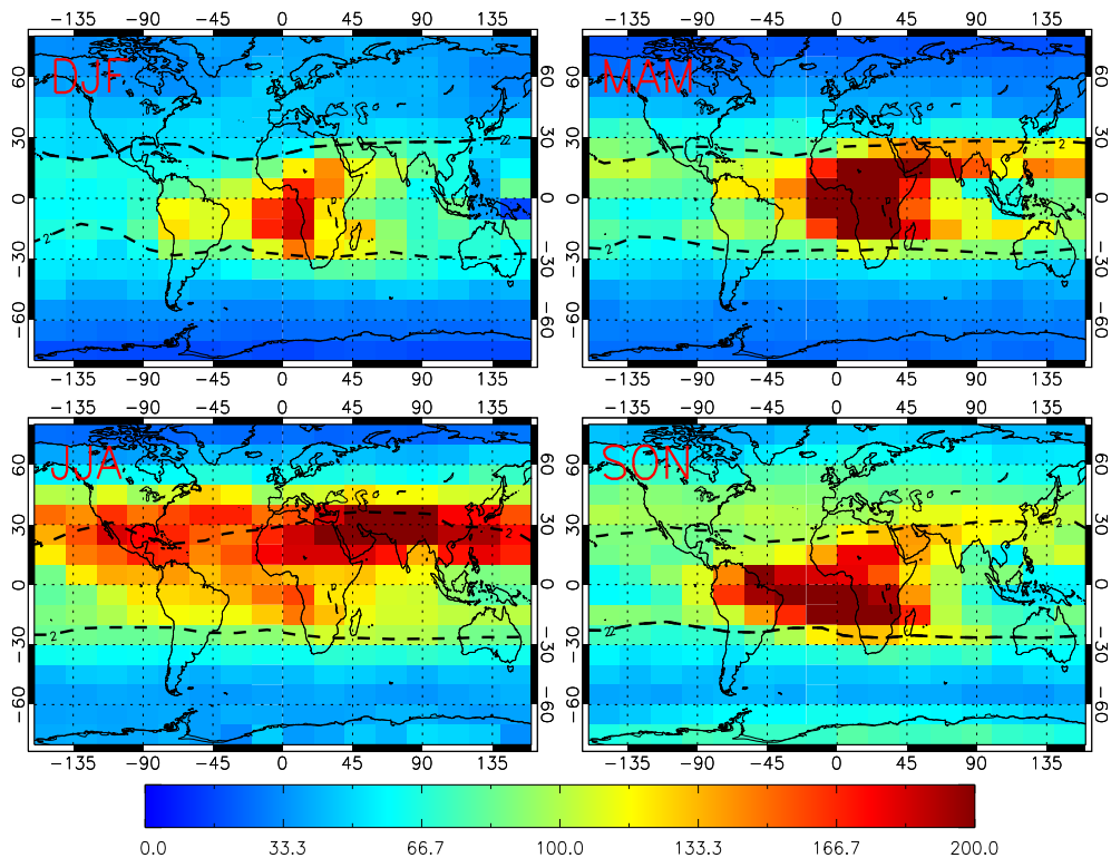
Fig. 2. MIPAS PAN (pptv) from the IMK retrieval at 150 hPa for 2007-2008 in December-January-February (DJF), March-April-May (MAM), June-July-August (JJA) and September-October-November (SON). The black dashed lines show the dynamical tropopause (defined as \pm 2 PVU) based on ERA-Interim data.
