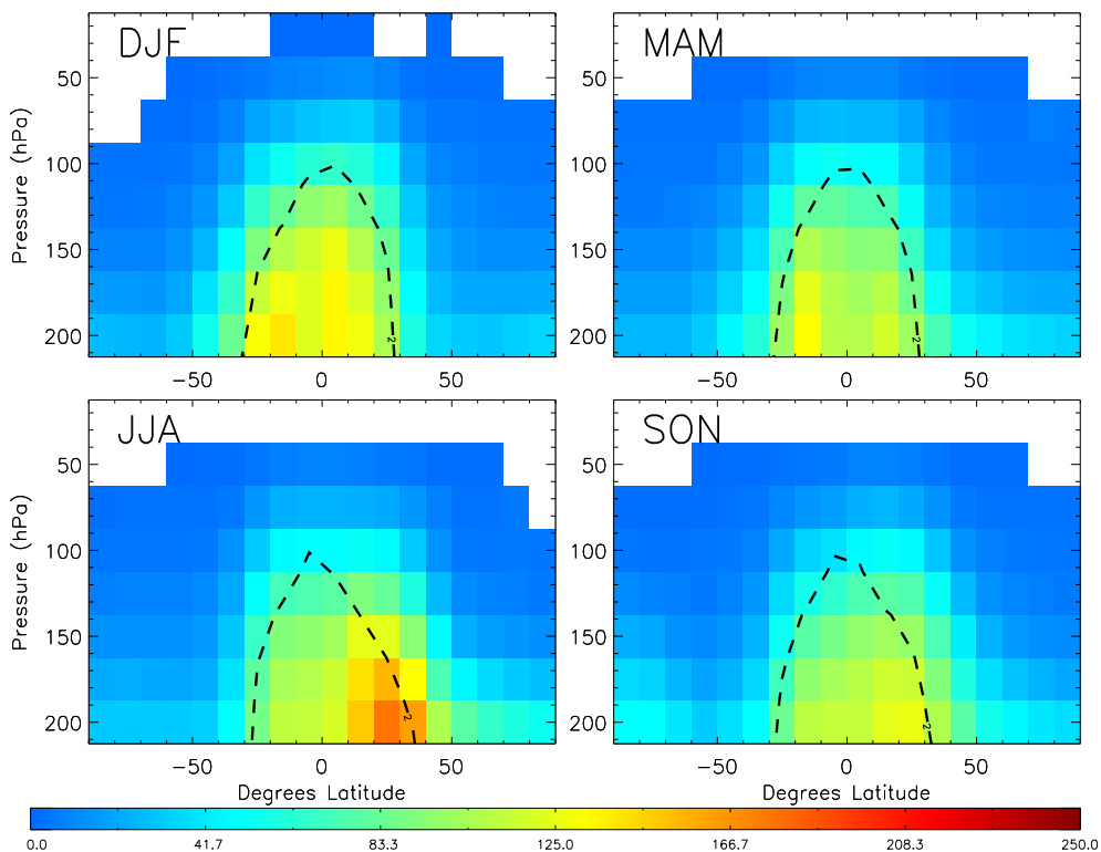
Fig. 14. Zonal mean PAN (pptv) from the TOMCAT model (with IMK AKs applied) for 2007-2008 in DJF, MAM, JJA and SON.
