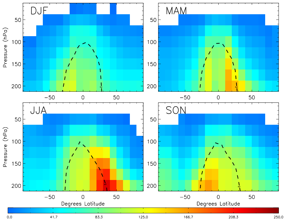
Fig. 5. Zonal mean MIPAS PAN (pptv) from the IMK retrieval for 2007-2008 in DJF, MAM, JJA and SON. The black dashed lines show the dynamical tropopause (defined as \pm 2 PVU) based on ERA-Interim data.
