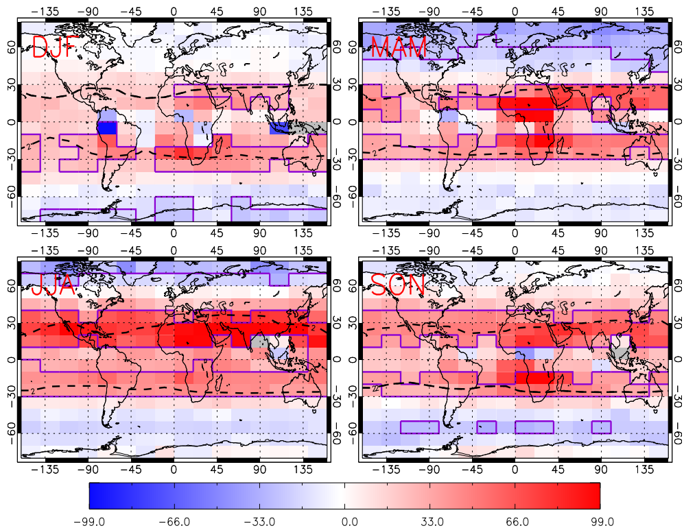
Fig. 4. Difference in MIPAS PAN (pptv) from IMK retrieval minus UoL retrieval at 150 hPa for 2007-2008 in DJF, MAM, JJA and SON. Purple polygonned regions show regions of significant differences, where the IMK and UoL retrieval uncertainty ranges do not overlap.
