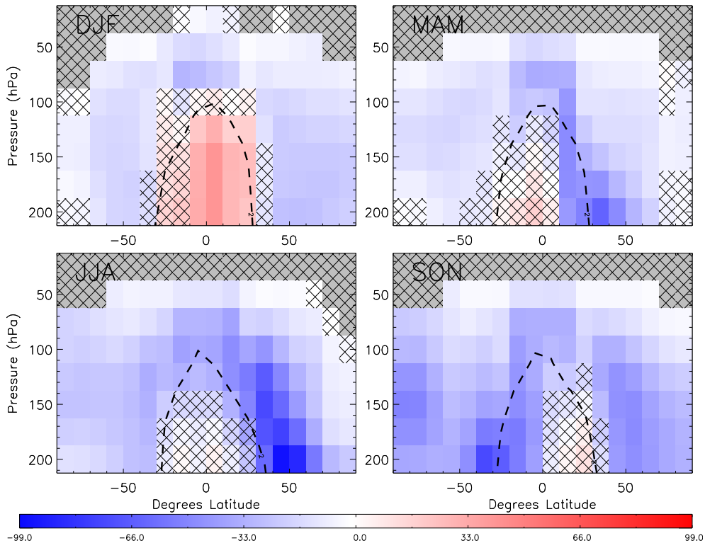
Fig. 16. Difference in zonal mean PAN (pptv) between the TOMCAT model (with IMK AKs applied) and observed IMK MIPAS PAN for 2007-2008 in DJF, MAM, JJA and SON. Hatching represents non-significant differences.
