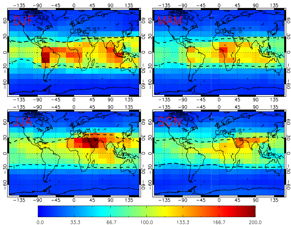
Fig. 10. Mixing ratio of PAN (pptv) from the TOMCAT model (with the IMK averaging kernels applied) at 150 hPa averaged over the periods DJF, MAM, JJA and SON in 2007-2008.
