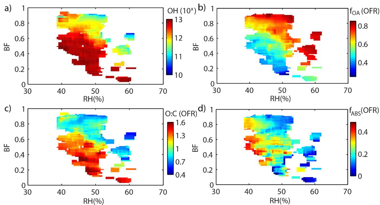
Figure 5. Scatterplot between BF, impactor RH and particle properties measured through the OFR; a) (RH,BF) –data colored with exposed OH concentration ( 10^x molec. \text{cm}^{-3} s), b) (RH,BF) –data colored with organic mass fraction of the particles derived from AMS results, c) (RH,BF) –data colored with O:C derived from AMS analysis, d) (RH,BF) –data colored with mass fraction of ammonium-bisulfate derived from AMS analysis and composition categorization as in Cerully et al. (2015). Data is filtered by precipitation < 1\text{mm h}^{-1} and ambient aerosols f_{\text{OA}} \geq 0.6 .
