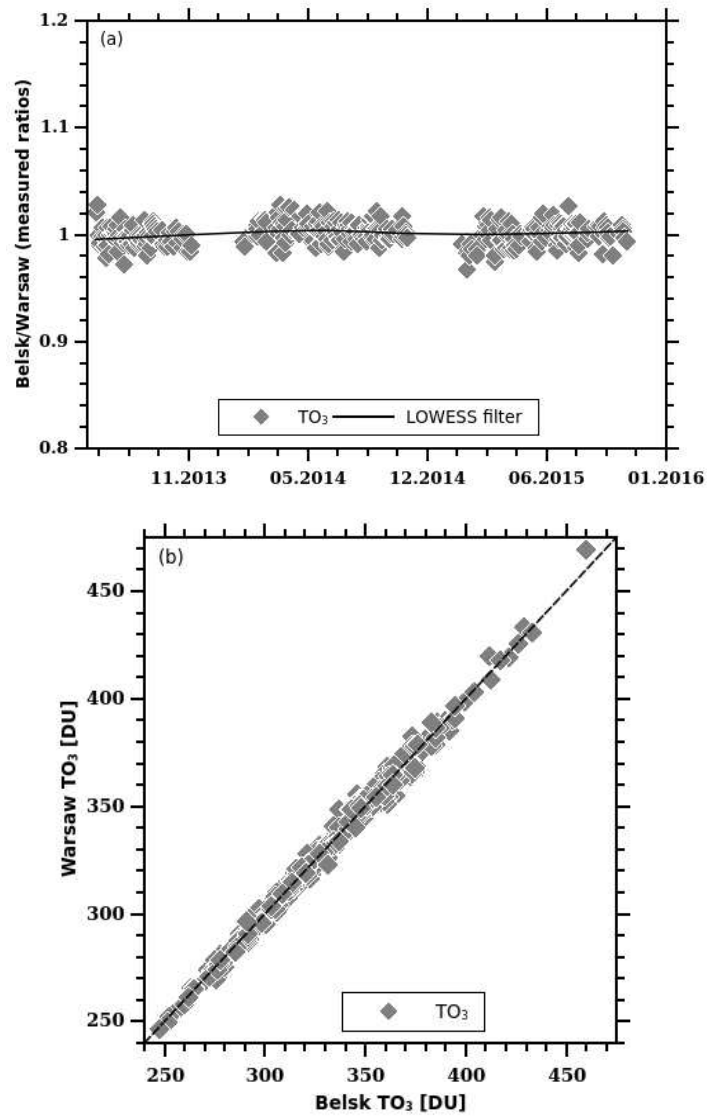
5 Figure 7a: The ratio between total ozone values measured by the Brewer Spectrophotometer No. 64 and No. 207 while working simultaneously at Belsk and in Warsaw for the period May 2013-December 2015. The solid curve represents the smoothed data by LOWESS filter.
