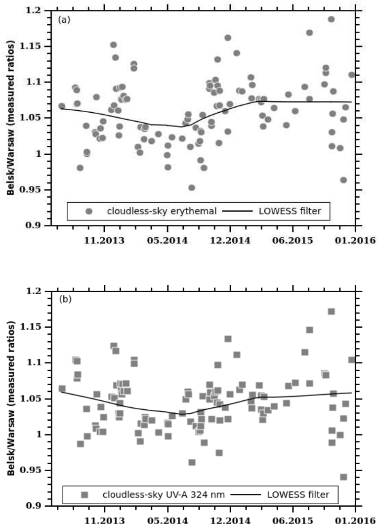
5 Figure 3: The Belsk/Warsaw ratio between the partial daily 3h doses (noon-3.5h, noon-0.5h) measured during cloudless-sky conditions existing over both sites for erythemal doses (a) and UV-A (324nm) doses (b). Solid curves represent the smoothed data by LOWESS filter.
