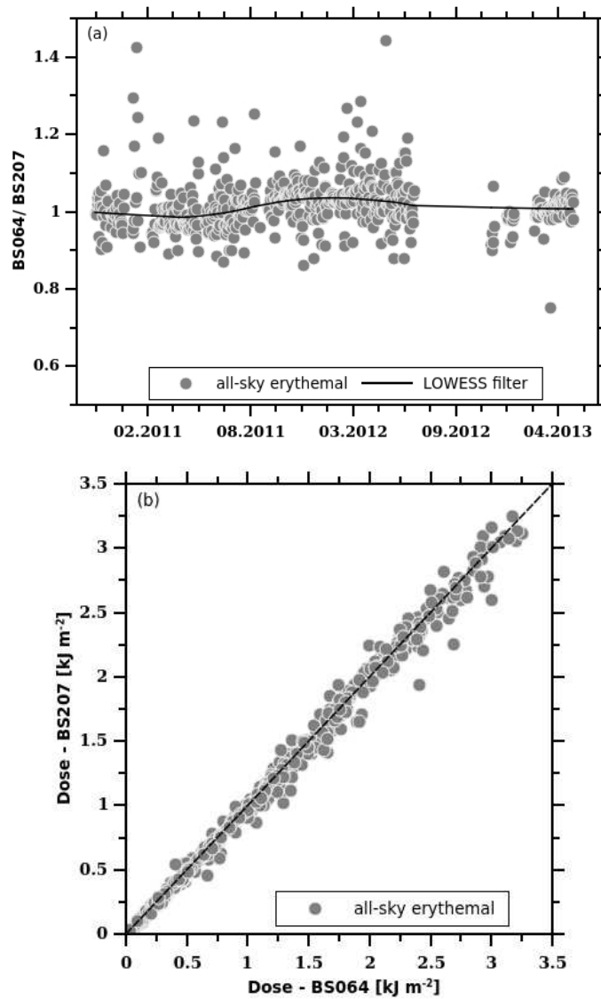
5 Figure 1a: The ratio between erythemal 6h (noon+/-3 hr) doses measured by the Brewer Spectrophotometer No. 64 and No. 207 while working simultaneously at Belsk (all-sky conditions). The solid curve represents the smoothed data by LOWESS filter.
