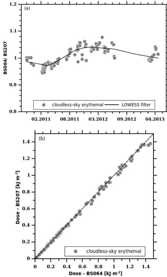
Figure 2a: Same as Fig.1a but for cloudless-sky conditions and 3h doses calculated for the period before noon (noon-3.5h, noon-0.5h).
