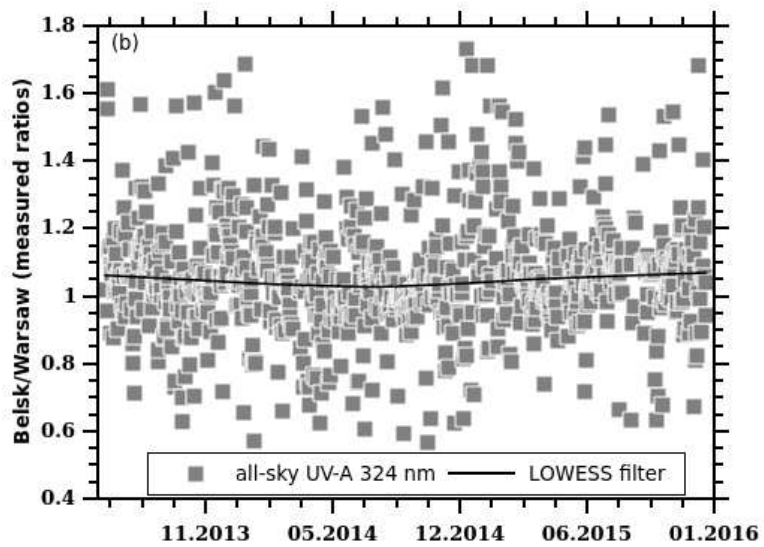
Figure 4: Same as Fig.5 but for the near noon partial daily dose (noon-3h, noon+3h) for all-sky conditions. Solid curves represent the smoothed data by LOWESS filter.
