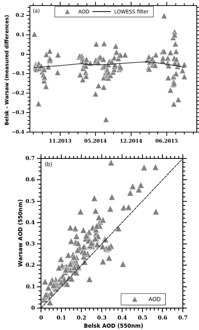
Figure 8a: The difference between AOD at 550nm measured simultaneously by MODIS over Belsk and Warsaw in the period May 2013-December 2015. The solid curve represents the smoothed data by LOWESS filter.
