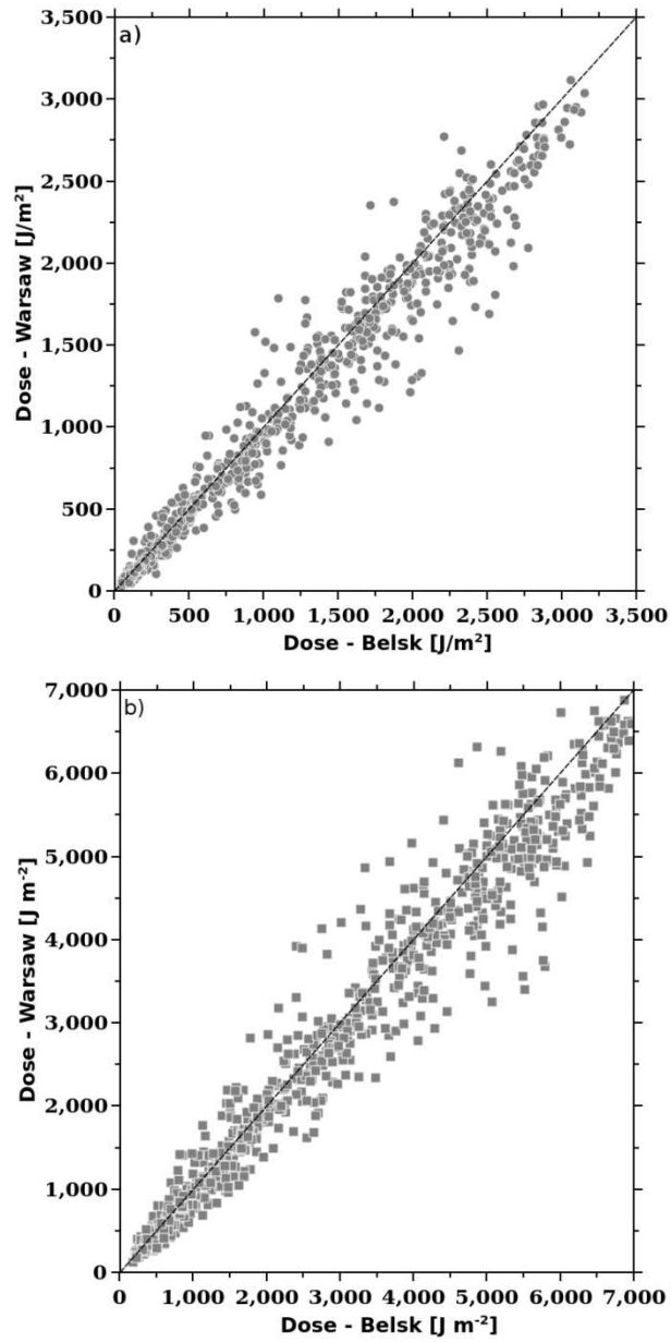
5 Figure 5: Scatter plot of partial daily doses (local noon-3h, local noon+3h) measured in Warsaw and Belsk: erythemal doses (a) and UV-A (324nm) doses (b).
