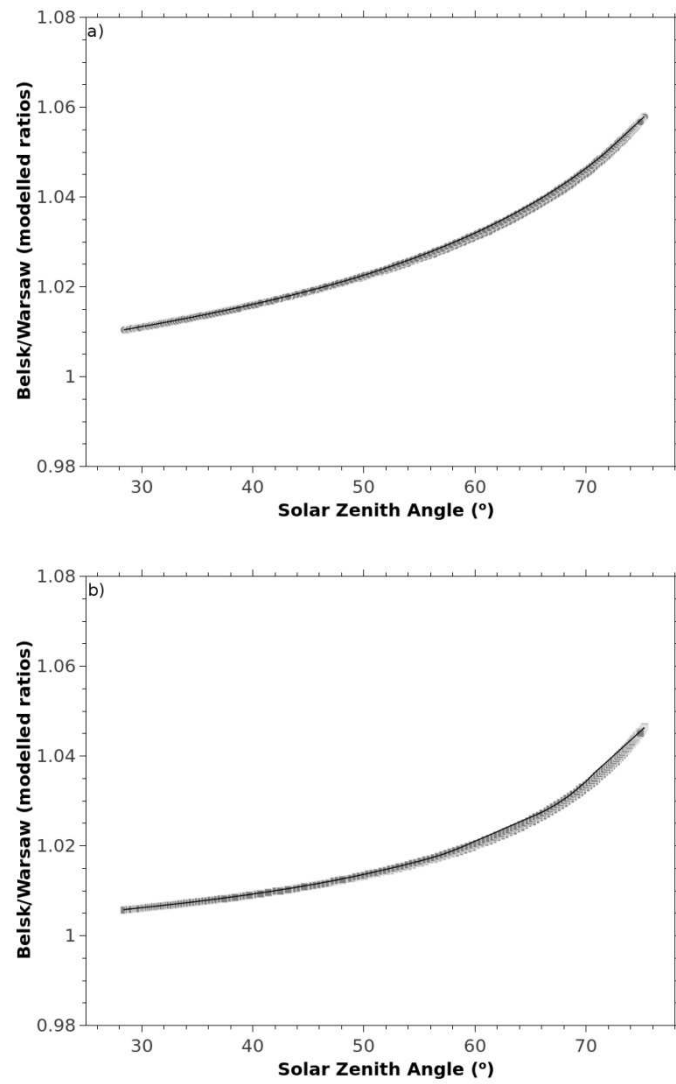
5 Figure 6: The Belsk/Warsaw ratio between erythemal (a) and UV-A (324nm) (b) irradiances calculated by the libRadtran model for 2015 versus SZA at Belsk for the 10:40 (GMT). The solid curve represents the smoothed data by LOWESS filter.
