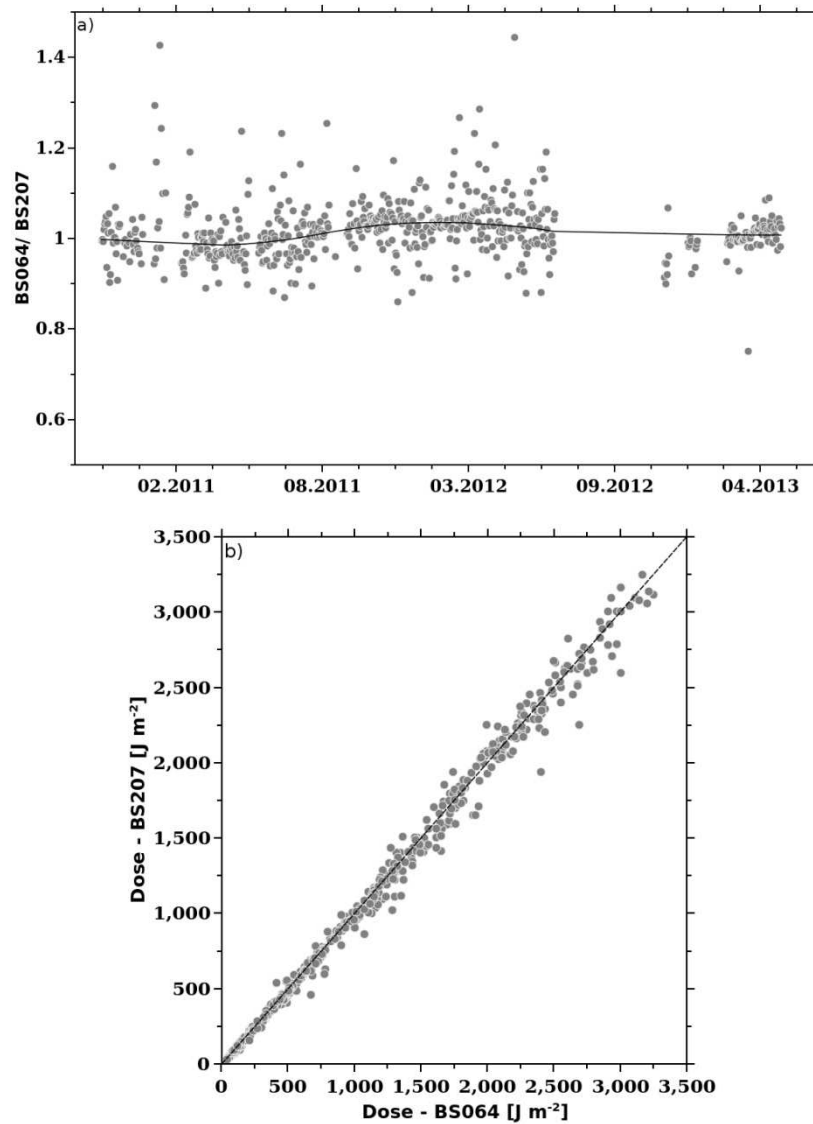
5 Figure 1a: The ratio between erythemal 6h (noon \pm 3 hr) doses measured by the Brewer Spectrophotometer No. 64 and No. 207 while working simultaneously at Belsk (all-sky conditions). The solid curve represents the smoothed data by LOWESS filter.
