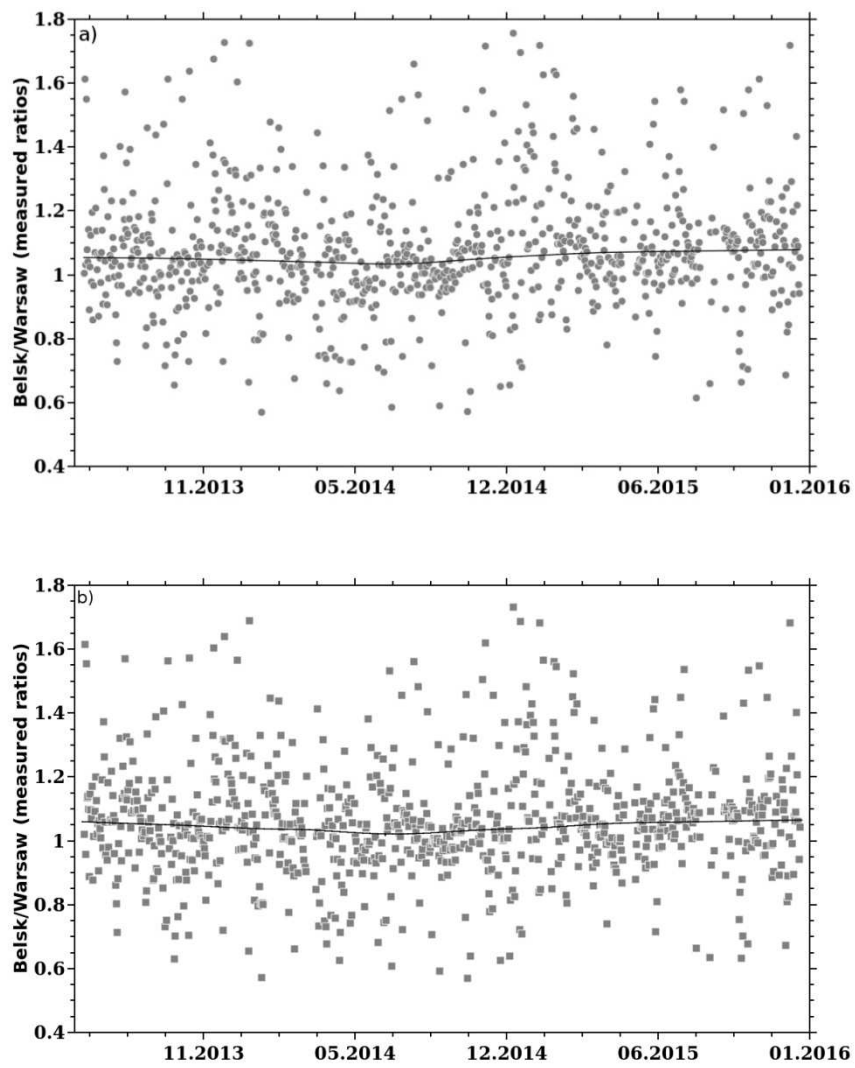
5 Figure 4: Same as Fig.5 but for the near noon partial daily dose (noon-3h, noon+3h) for all-sky conditions. Solid curves represent the smoothed data by LOWESS filter.
