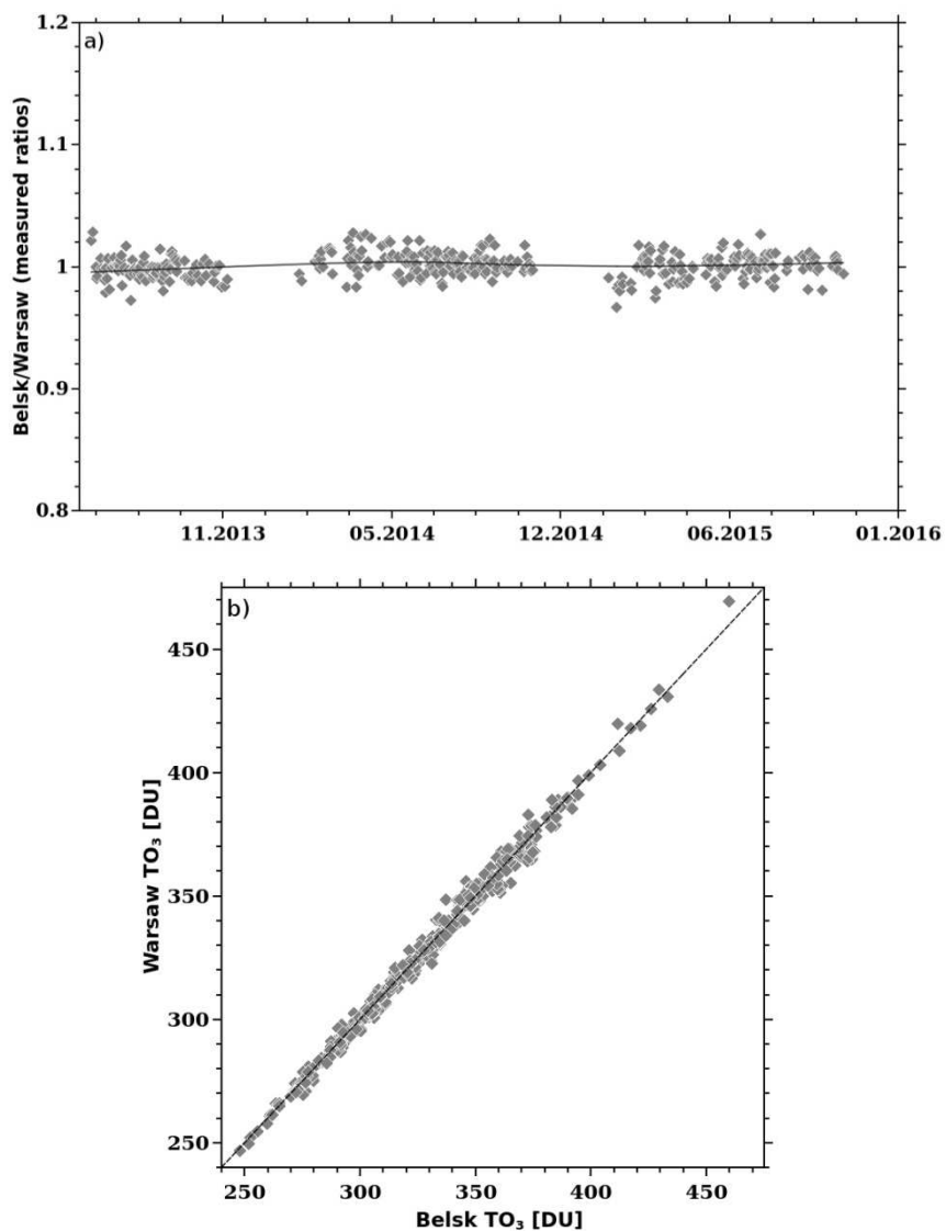
5 Figure 7a: The ratio between total ozone values measured by the Brewer Spectrophotometer No. 64 and No. 207 while working simultaneously at Belsk and in Warsaw for the period May 2013-December 2015. The solid curve represents the smoothed data by LOWESS filter.
