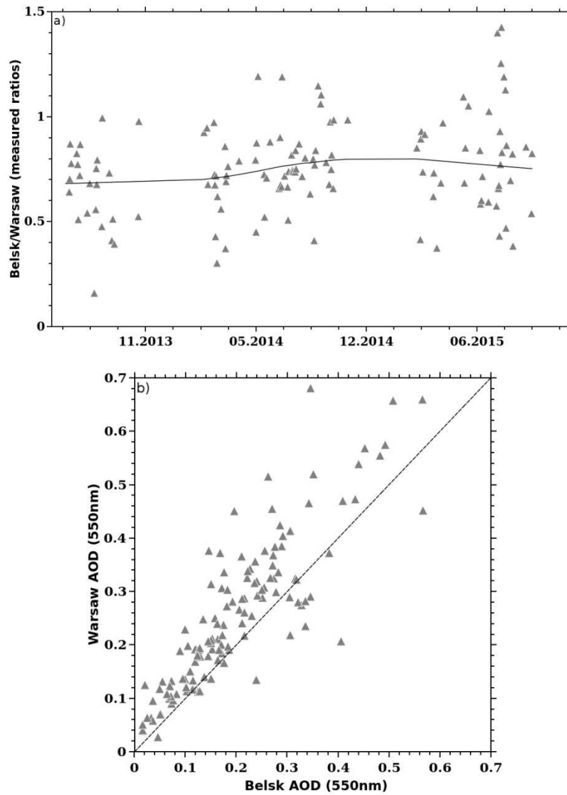
Figure 8a: The ratio between AOD at 550nm measured simultaneously by MODIS over Belsk and Warsaw in the period May 2013-December 2015. The solid curve represents the smoothed data by LOWESS filter.
