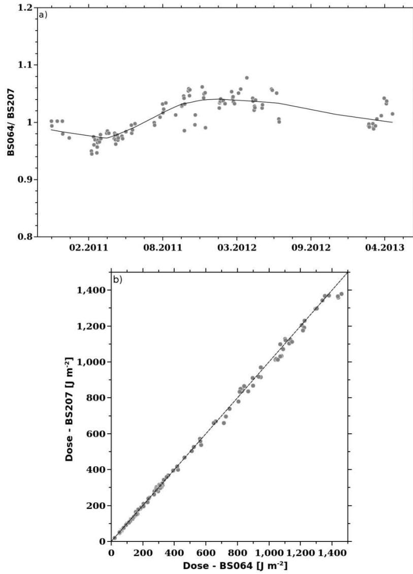
5 Figure 2a: Same as Fig.1a but for cloudless-sky conditions and 3h doses calculated for the period before noon (noon-3.5h, noon-0.5h).
