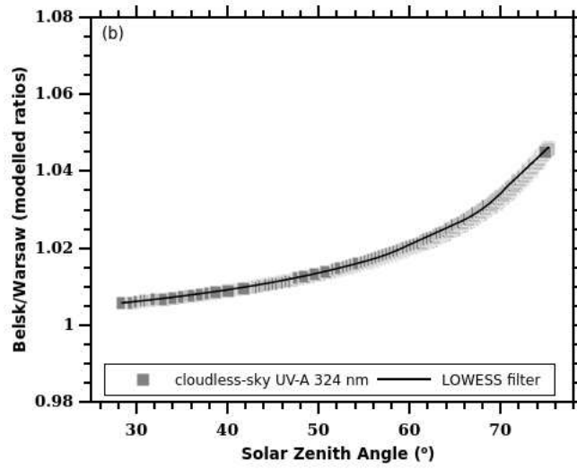
Figure 6: The Belsk/Warsaw ratio between erythemal (a) and UV-A (324nm) (b) irradiances calculated by the libRadtran model for 2015 versus SZA at Belsk for the 10:40 (GMT). The solid curve represents the smoothed data by LOWESS filter.
