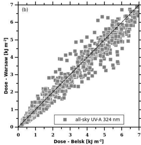
5 Figure 5: Scatter plot of partial daily doses (local noon-3h, local noon+3h) measured in Warsaw and Belsk: erythemal doses (a) and UV-A (324nm) doses (b).
