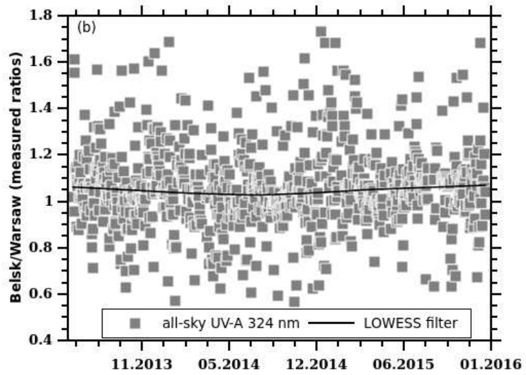
5 Figure 4: Same as Fig.5 but for the near noon partial daily dose (noon-3h, noon+3h) for all-sky conditions. Solid curves represent the smoothed data by LOWESS filter.
