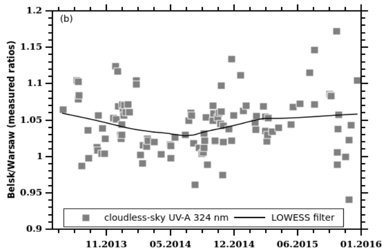
Figure 3: The Belsk/Warsaw ratio between the partial daily 3h doses (noon-3.5h, noon-0.5h) measured during cloudless-sky conditions existing over both sites for erythemal doses (a) and UV-A (324nm) doses (b). Solid curves represent the smoothed data by LOWESS filter.
