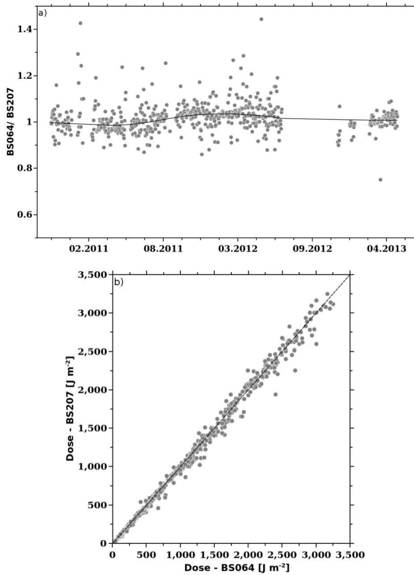
5 Figure 1a: The ratio between erythemal 6h (noon \pm 3 hr) doses measured by the Brewer Spectrophotometer No. 64 and No. 207 while working simultaneously at Belsk (all-sky conditions). The solid curve represents the smoothed data by LOWESS filter.
