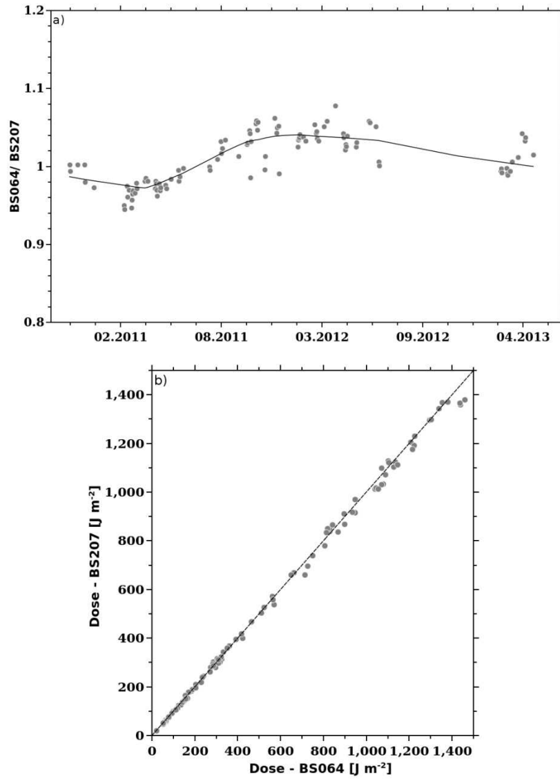
Figure 2a: Same as Fig.1a but for cloudless-sky conditions and 3h doses calculated for the period before noon (noon-3.5h, noon-0.5h).
