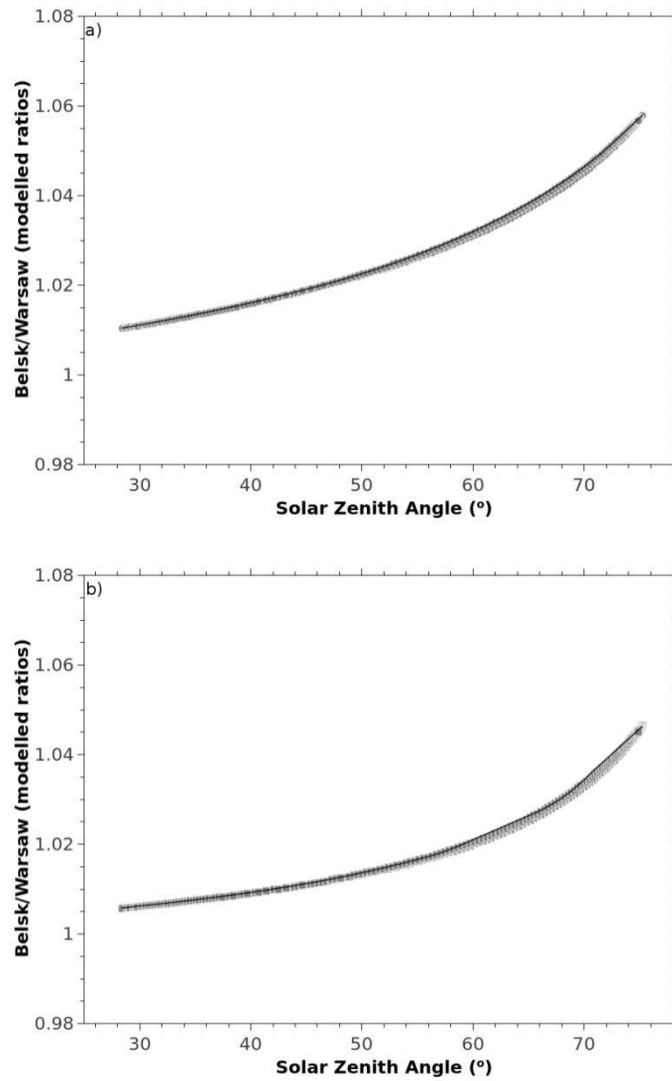
5 Figure 6: The Belsk/Warsaw ratio between erythemal (a) and UV-A (324nm) (b) irradiances calculated by the libRadtran model for 2015 versus SZA at Belsk for the 10:40 (GMT). The solid curve represents the smoothed data by LOWESS filter.
