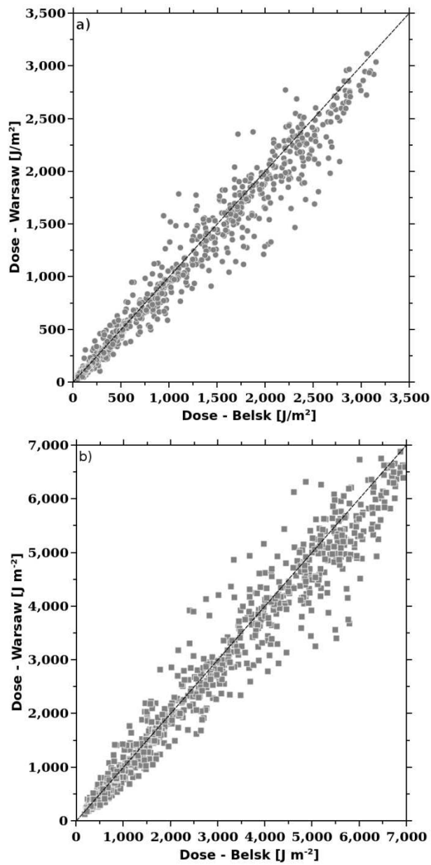
Figure 5: Scatter plot of partial daily doses (local noon-3h, local noon+3h) measured in Warsaw and Belsk: erythemal doses (a) and UV-A (324nm) doses (b).
