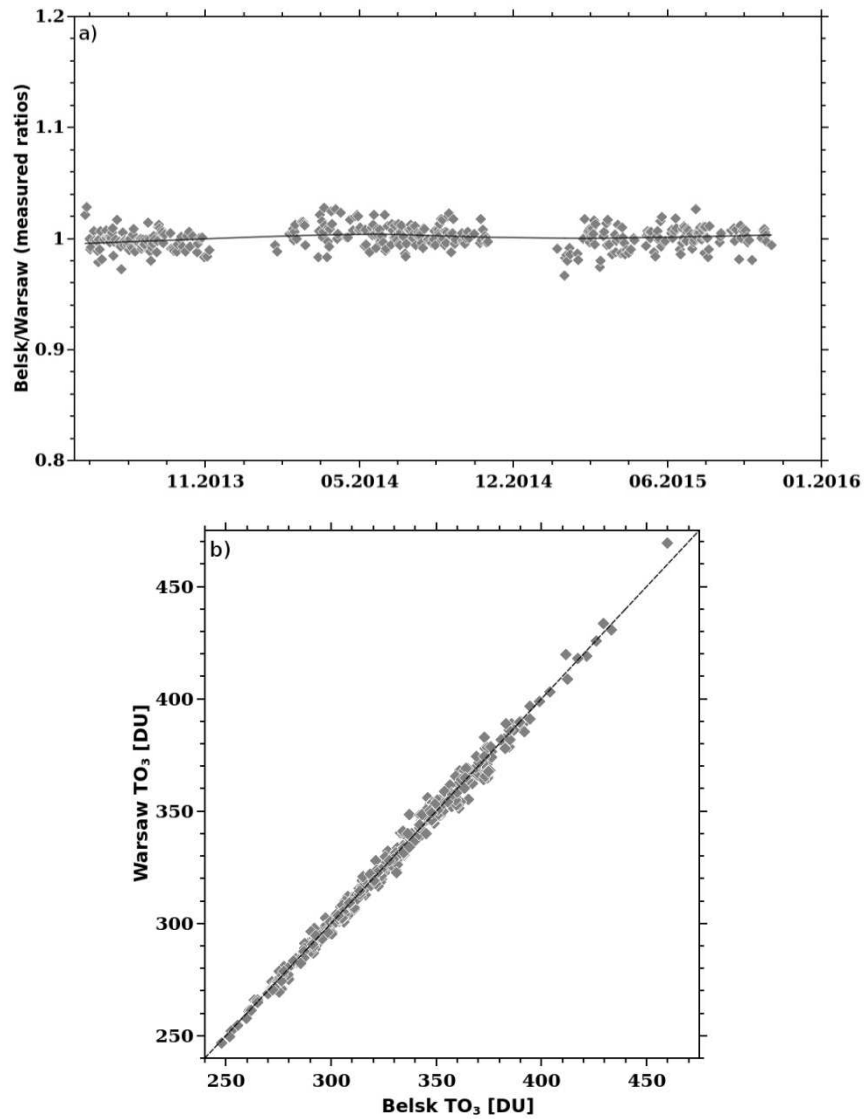
Figure 7a: The ratio between total ozone values measured by the Brewer Spectrophotometer No. 64 and No. 207 while working simultaneously at Belsk and in Warsaw for the period May 2013-December 2015. The solid curve represents the smoothed data by LOWESS filter.
