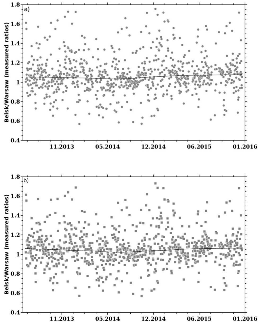
Figure 4: Same as Fig.5 but for the near noon partial daily dose (noon-3h, noon+3h) for all-sky conditions. Solid curves represent the smoothed data by LOWESS filter.
