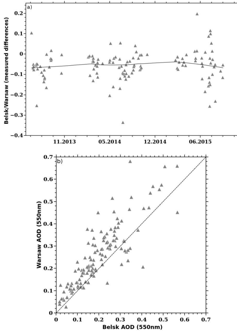
Figure 8a: The difference between AOD at 550nm measured simultaneously by MODIS over Belsk and Warsaw in the period May 2013-December 2015. The solid curve represents the smoothed data by LOWESS filter.
