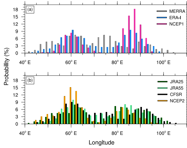
Figure 6. As Fig. ??-5 but for monthly mean data. Additionally the original distribution has been smoothed using a running average over three grid points (JJA 1979–2014 7.5°).
