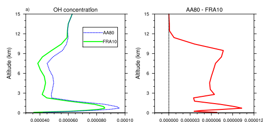
Figure 16: Vertical profiles of OH (in \mu\text{g}/\text{m}^3 ) for the FRA10 and AA80 simulations and the differences between them. FRA10 simulations are in green, the AA80 in dashed blue and the differences in red.
