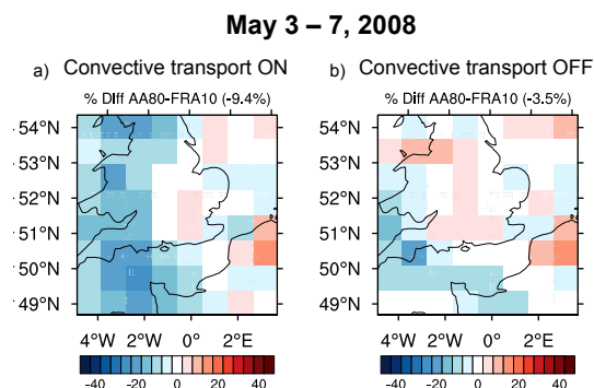
Figure 11: Percent differences in mean spatial distribution of column amount of accumulation mode aerosol water content (in \mu\text{g m}^{-2} ) between the FRA10 and AA80 simulations for the period of May 3 - 7, 2008, with convective transport turned on (a) and turned off (b).
