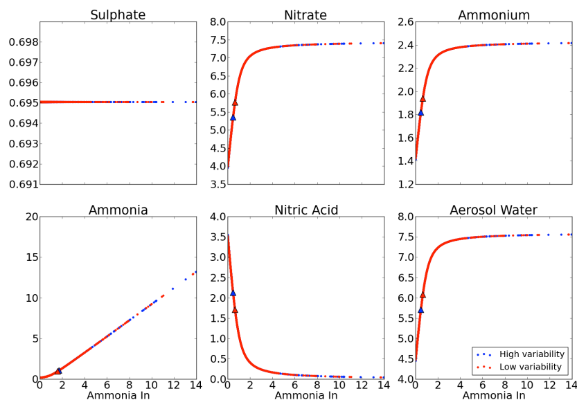
Figure 7: Example of sensitivity test where input ammonia concentrations are randomly sampled at high (blue) and low (red) variability (RH = 0.70, temperature = 280K). The subplots show the equilibrium concentrations (in \mu\text{g m}^{-3} ) of individual aerosol/gaseous species as a function of input ammonia concentrations. The blue and red triangles represent the mean equilibrium concentrations of the aerosol/gaseous species in the high and low variability runs.
