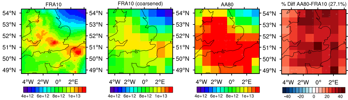
Figure 13: Spatial distribution of column amount of accumulation mode number concentration ( \# \text{m}^{-2} ) for the FRA10 simulation, the FRA10 simulation coarsened to the low resolution grid, the AA80 simulation, and the percent difference between the two. The number in brackets on the third panel represents the average percentage difference in the two runs.
