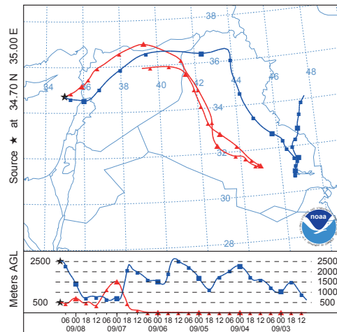
Figure 3. Six-day HYSPLIT backward trajectories ( http://www.arl.noaa.gov/HYSPLIT.php ) arriving in the Cyprus region at 35°E (about 160 km east of the Limassol lidar station) at 500 m (red, lower dust layer) and 2500 m height (blue, upper dust layer) on 8 September 2015, 09:00 UTC (12:00 EEST).
