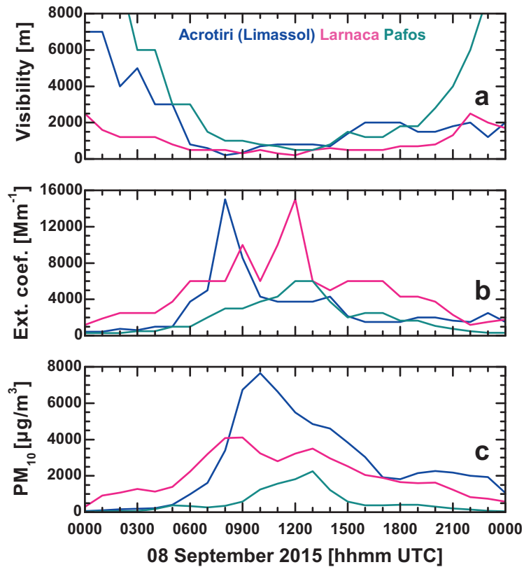
Figure 8. Visibility ( r_{vis} in Eq. (2)) measured at three airports in southern Cyprus (see map in Fig. 7c) on 8 September 2015, (b) corresponding dust extinction coefficient (by using Eq. (2)), and (c) PM_{10} concentrations (same as shown in Fig. 7c). Relative uncertainties in all parameters are of the order of 50%. Dust extinction coefficients of 4000\text{--}8000\text{ Mm}^{-1} indicate dust mass concentrations of 6600\text{--}13300\ \mu\text{g}/\text{m}^3 .
