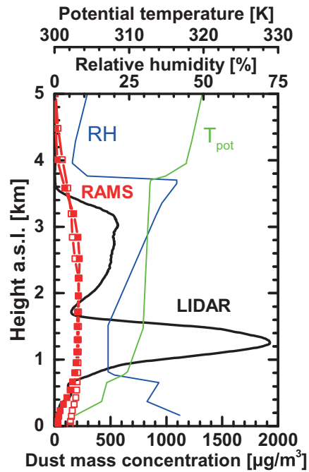
Figure 5. Mean dust mass concentration observed with lidar (thick solid black line) at Limassol on 7 September, 19:00–20:00 UTC , and dust profiles simulated with RAMS (normal run with 20 km horizontal resolution) for Limassol, on 7 September, 18:00 UTC (closed red squares), and 8 September, 9:00 UTC (open squares). Radiosonde observation (launched at the radiosonde station at Athalassa near Nicosia on 8 September 6:00 UTC) of height profiles of potential temperature ( T_{pot} , thin green curve) and relative humidity (RH, thin blue curve) are in good agreement with the two-layer dust structures observed about 12 hours earlier. The lofted dust layer from 1.7–3.6 km height was well mixed.
