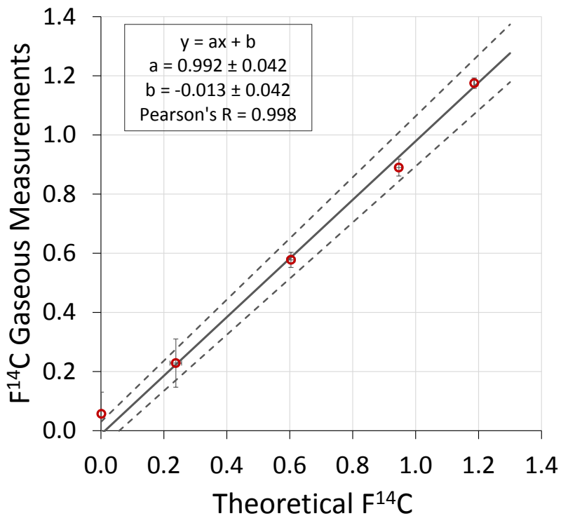
5 Figure 2: F^{14}C values of synthetic and standard (test) aerosol samples measured with the gas source compared with theoretical values. These test aerosols are made of two Standard Reference Materials (SRM 2975 and SRM 1515). The compositions of the different mixtures are listed in Table 1 with the corresponding theoretical and measured F^{14}C . The coefficients of the linear regression have been calculated by taking into account error bars (2 SD) on both axes and are given with their 95 % confidence interval. The linear relation confirms the accuracy of aerosol measurements with the gas ion source over the full range of expected ^{14}C activities.
