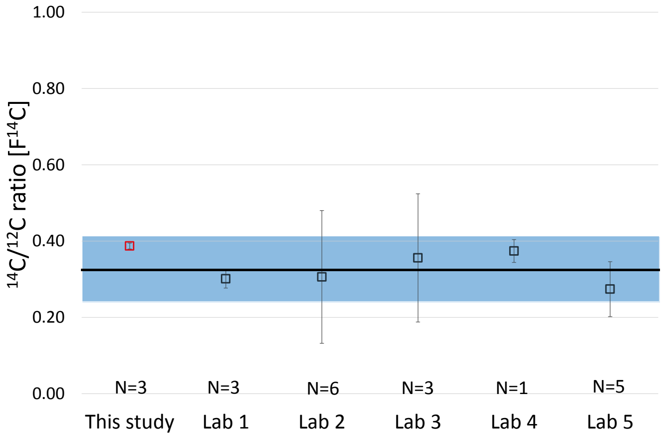
5 Figure 3: RM 8785 measurements. Black squares and error bars represent values and measurement uncertainties at 2\sigma , described in Szidat et al. (2013). The black line stands for the average value and the blue ribbon represents the 2\sigma confidence interval for Labs 1-5. The red square shows the weighted average result obtained for this study ( N = 3 ) and its weighted error ( 2\sigma ). The large scatter could be linked to heterogeneous loading during the production of RM 8785 as mentioned by Cavanagh and Watters (2005). The value obtained in this study is compatible with the high end of measurements performed by the five different laboratories.
