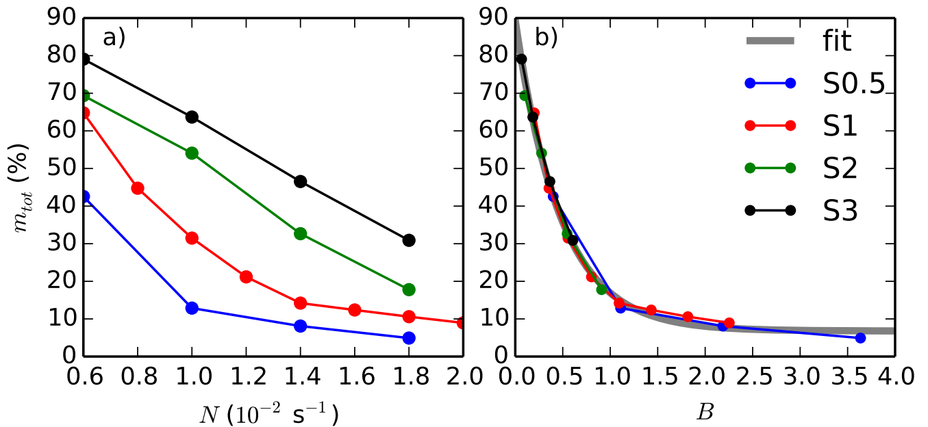
Figure 8. Total tracer mass exported out of the valley atmosphere at crest height normalized by the total tracer mass released at the surface as a function of (a) Brunt-Väisälä frequency and (b) breakup parameter for various different forcing amplitudes. A fit to the data according to Eq. 10 is shown in (b).
