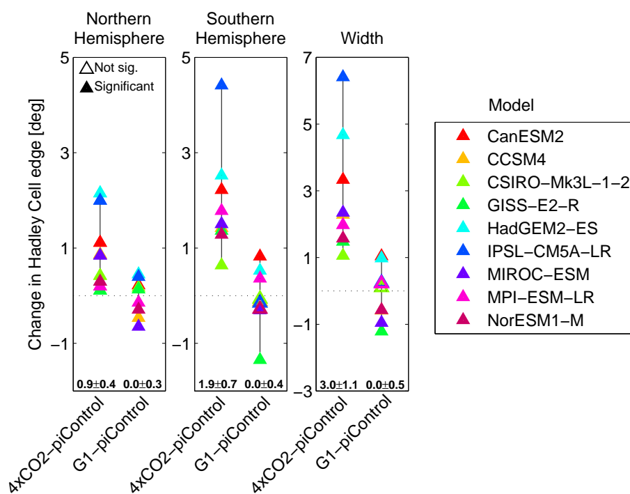
Figure 4. The change in the Hadley cell edge latitudes and width between the 4×CO 2 and piControl experiments and between the G1 and piControl experiments, for the Northern Hemisphere and Southern Hemisphere edge latitudes and for the total change in Hadley cell width (Width). Positive values indicate poleward expansion or an increase in width. Models with edge latitude or width changes significant at the 95% confidence level are indicated by solid symbols. The mean change in the tropical belt width or edge latitude and its 95% confidence interval in degrees latitude is shown at the bottom of each plot.
