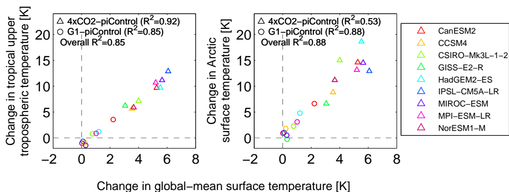
Figure 10. The change in tropical upper-tropospheric temperature versus the change in global-mean surface temperature (left), and the change in Arctic surface temperature versus the change in global-mean surface temperature (right), between the 4\times\text{CO}_2 and piControl experiments (triangles) and between the G1 and piControl experiments (circles). Tropical upper-tropospheric temperature is defined as the mean temperature between 200 and 300 hPa and between 10S and 10N. Arctic temperature is defined as the mean surface temperature between 75N and 90N.
