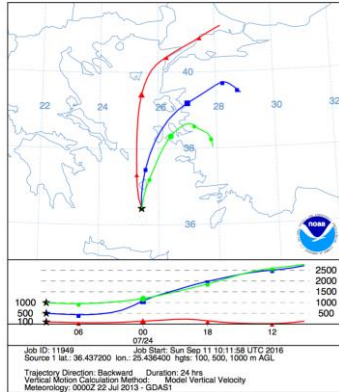
NOAA HYSPLIT MODEL Backward trajectories ending at 0900 UTC 24 Jul 13 GDAS Meteorological Data
