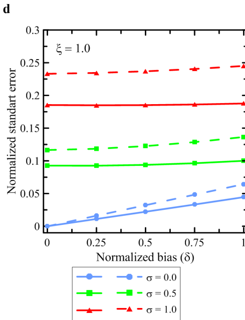
Figure 7: The same as in and Fig. 6 but for the dependencies of the normalized standard error on the scaling factor, \delta , characterizing the bias applied to the synthetic data (see Sect. 3.5 for further details).
