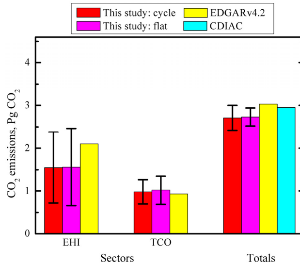
Figure 11: Hybrid estimates of the fossil-fuel CO 2 emissions measurements ( \hat{E}_{sc}^{co2} , \hat{E}_{s,tot}^{co2} , \hat{E}_{comb,c}^{co2} and \hat{E}_{comb,tot}^{co2} ) from the study region in comparison with the data of the EDGAR v4.2 and CDIAC emission inventories. The estimates were obtained either from (a) only NO x and (b) only CO or (c) from both NO x and CO measurements. The "partial" and "full" 68.3% confidence intervals are also shown: the "partial" intervals (depicted by narrow brackets and not shown for the combined CO 2 emission estimates) are determined only by uncertainties in the top-down estimates of NO x or CO emissions, while the "full" intervals take into account also probable uncertainties in the conversion factors.
