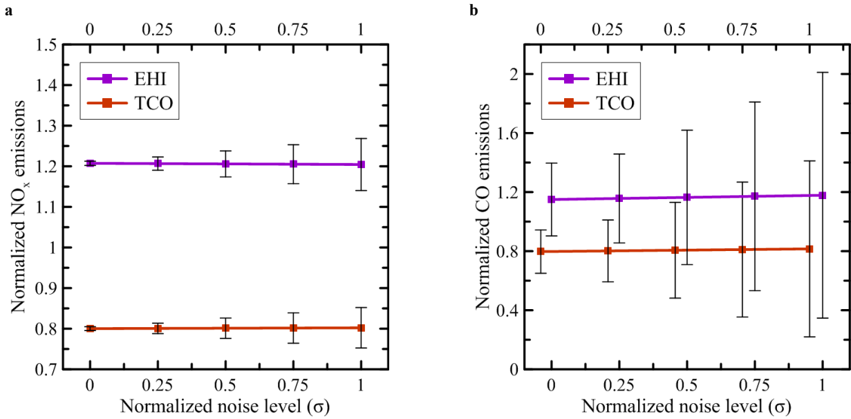
Figure 9: The NO x (a) and CO (b) emission estimates obtained similar to the estimates shown in Fig. 8 but separately for the two source categories (EHI and TCO) in the OSSEs where the "true" emissions in the EHI and TCO were specified by scaling the corresponding bottom-up emissions (employed in the base case model run) with the factors of 1.2 and 0.8. Note that the estimates for the EHI and TCO categories are depicted by using the abscissa axes at the bottom and at the top of the plots, respectively.
