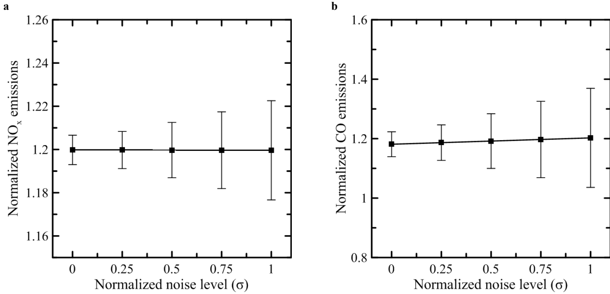
Figure 8: The total \text{NO}_x (a) and CO (b) emission estimates ( \hat{E}_{tot}^s ) obtained in the OSSEs where the "true" emissions were specified by scaling the bottom-up emissions (employed in the base case model run) with the factor of 1.2. The emission estimates (normalized to the respective bottom-up emission estimates, \tilde{E}_{tot}^s , based on the EMEP inventory data) represent the average over the ensemble of 100 Monte Carlo experiments, each with a different sample of noise in the synthetic data, and are shown as a function the noise level ( \sigma ). Both non-diagonal elements of the error co-variance matrix and the systematic uncertainties were taken into account in the OSSEs (specifically, both \xi and \delta were set to be equal to unity, see further details in Sect. 3.5). Note that the value of 1.2 on the axis of ordinates corresponds to a perfect emission estimate in the case considered. Note also that the confidence intervals shown were estimated by using the subsampling technique (see Eq. 12) that is expected to predict a non-zero uncertainty (associated with the bias estimation procedure) even when the synthetic input data are not affected by random uncertainties (that is, when \sigma=0 , see also blue lines in Fig. 7).
