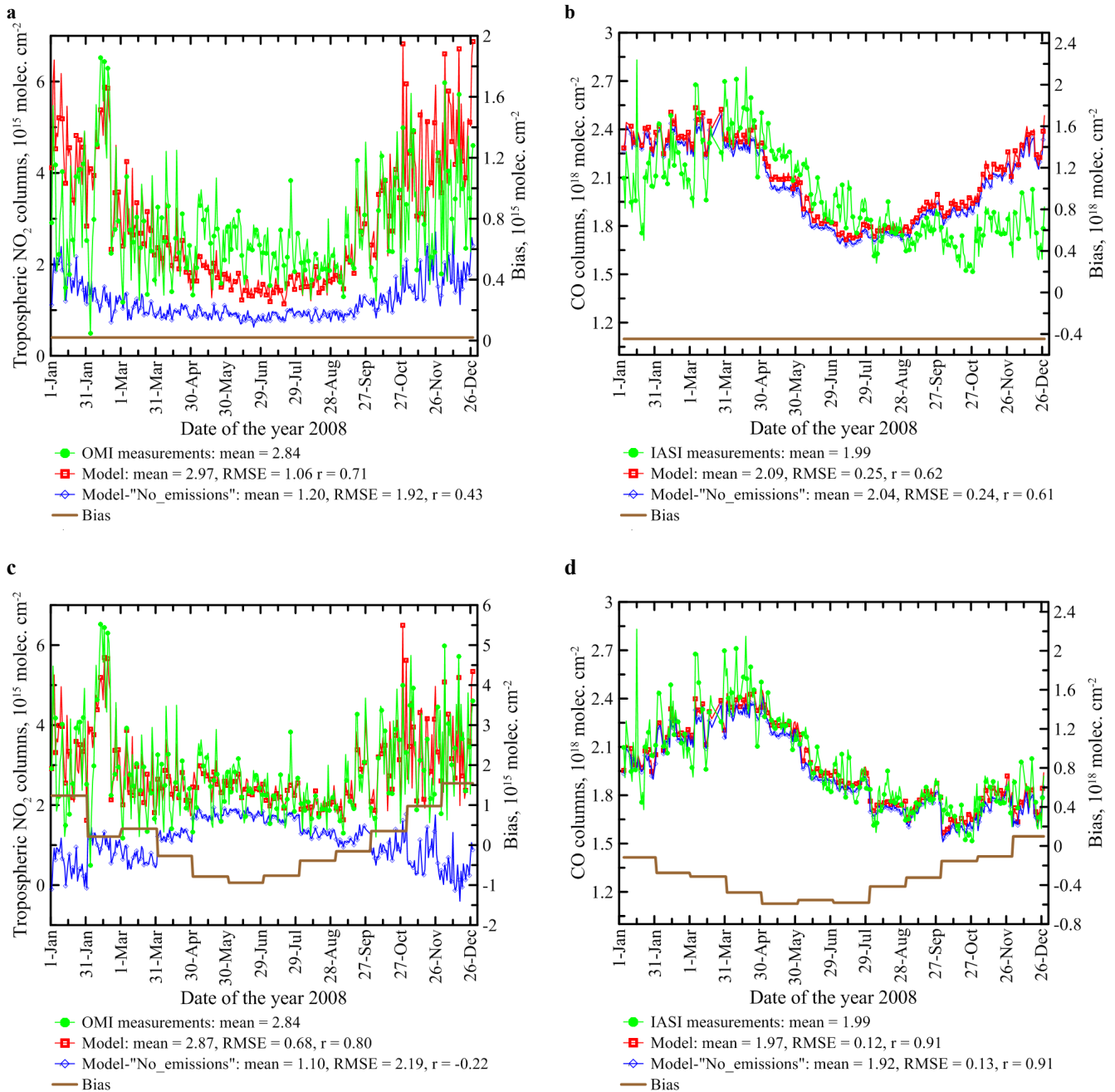
Figure 3: Time series of the spatially-averaged \text{NO}_2 (a,c) and CO (b,d) columns retrieved from satellite measurements (see green curves) and simulated using the CHIMERE CTM both with and without anthropogenic emissions in the study region (see red and blue curves, respectively). The simulated data shown have been de-biased: the differences (see brown curves) between either the annual (a,b) or monthly (c,d) averages of the simulation and measurement data were subtracted from the original simulation data.
