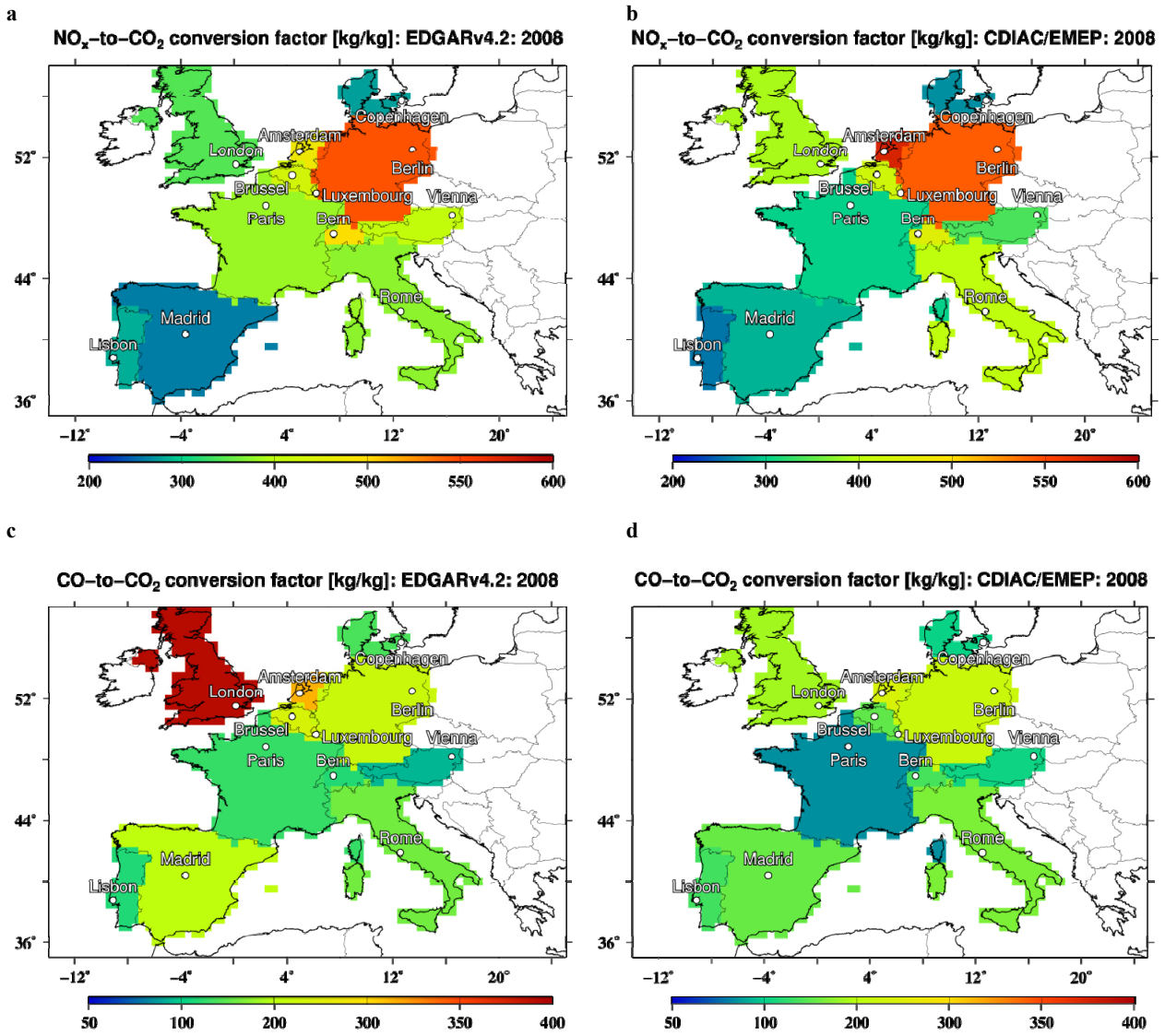
Figure 5: \text{NO}_x -to- \text{CO}_2 (a, b) and \text{CO} -to- \text{CO}_2 (c, d) emission conversion factors obtained using \text{NO}_x , \text{CO} , and \text{CO}_2 emission estimates from the EDGAR v4.2 emission inventory (a, c) and from the CDIAC and EMEP emission inventories (b, d) for the emission totals.
