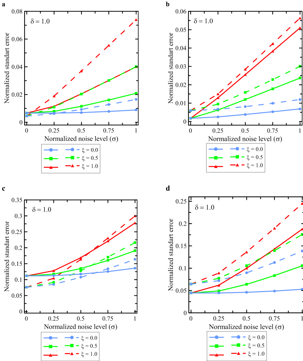
Figure 6: Results of the OSSEs for estimation of \text{NO}_x (a,b) and CO (c,d) emissions: the dependencies of the normalized standard error of the \text{NO}_x (CO) emission estimates for the EHI (a,c) and TCO (b,d) source categories on the level of noise (that is, on the value of the diagonal elements, \sigma , of the error covariance matrixes) in the input "synthetic" data. The noise level is normalized to its magnitude estimated with the real measurement and simulation data. Apart from the random noise, the synthetic data included the bias that was specified (for any given day) by linearly interpolating (in time) the monthly biases shown in Fig. 3(c,d). Different colors show the results obtained with the different levels of error co-variances ( \xi is the scaling factor applied to non-diagonal elements of the covariance matrix). The standard errors estimated in the "direct" way (as the RMSE representing the differences between the emission estimates inferred from the synthetic data and the "true" \text{NO}_x emission estimates) and by using the subsampling technique are shown by solid and dashed lines, respectively.
