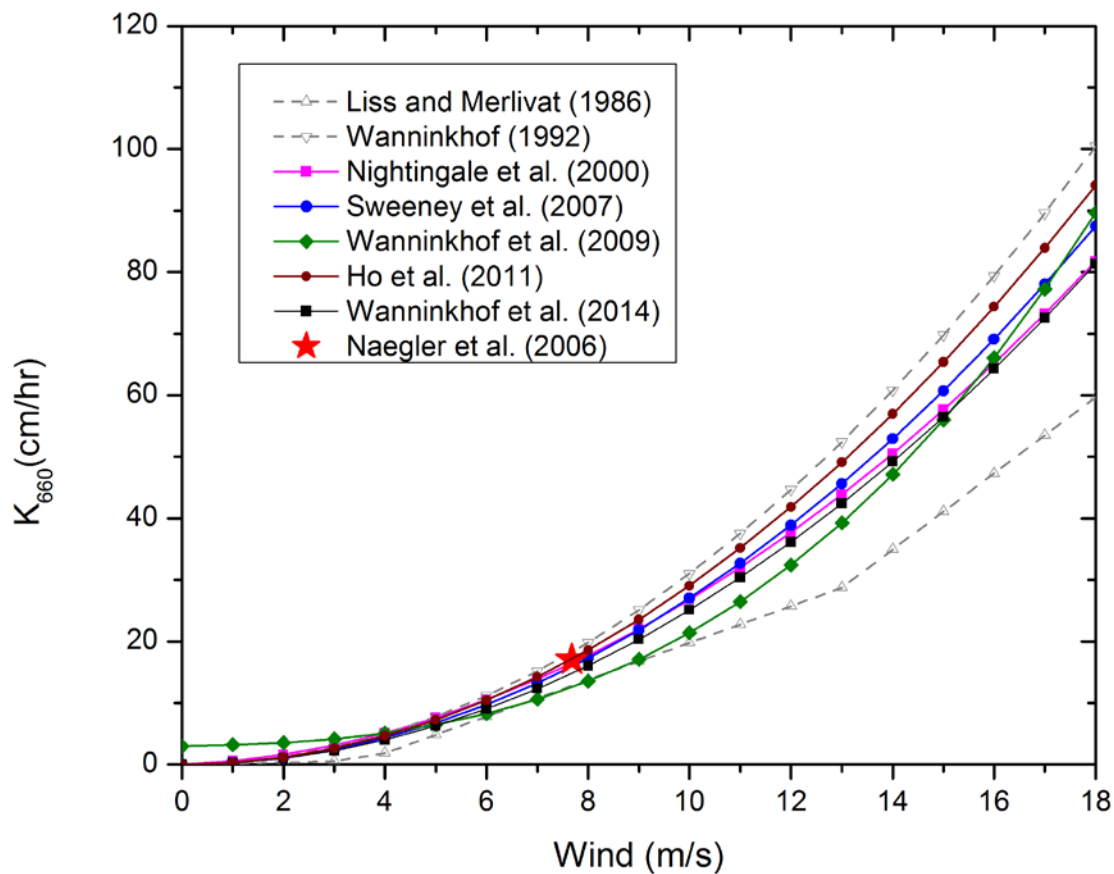
Figure 8. Various wind speed relationships for the air sea exchange velocity ( K_{w,660} ) determined in previous studies. Curves from each of these studies were normalized to \text{CO}_2 , but as shown here, have been adjusted to represent \text{CCl}_4 according to its Schmidt number, which, a function of viscosity of the medium and diffusivity of the gas, is largely a function of sea surface temperature.
