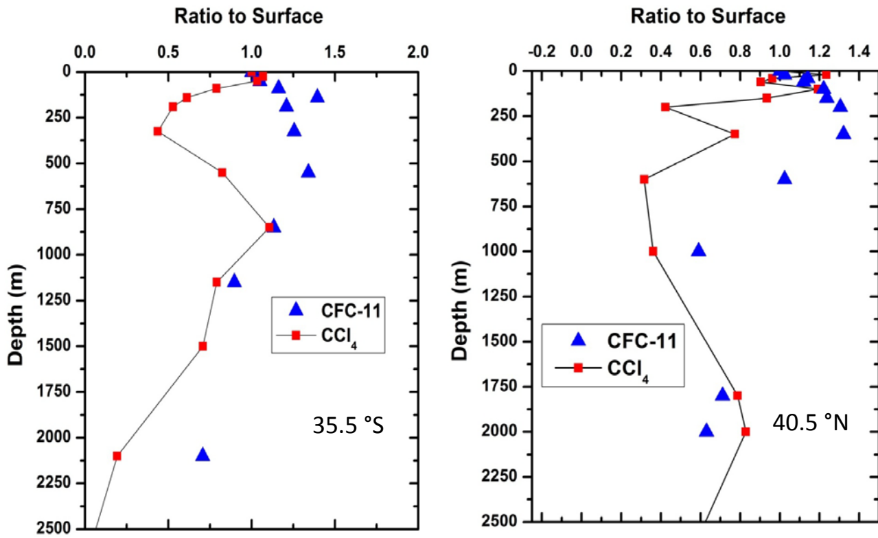
5 Figure 6. Depth profiles of the concentrations of CCl 4 and CFC-11, normalized to the surface value, strongly suggest consumption of CCl 4 in intermediate waters. If there were no in situ consumption and the distributions entirely a function of mixing and transport, the curves would be similar if not identical.
