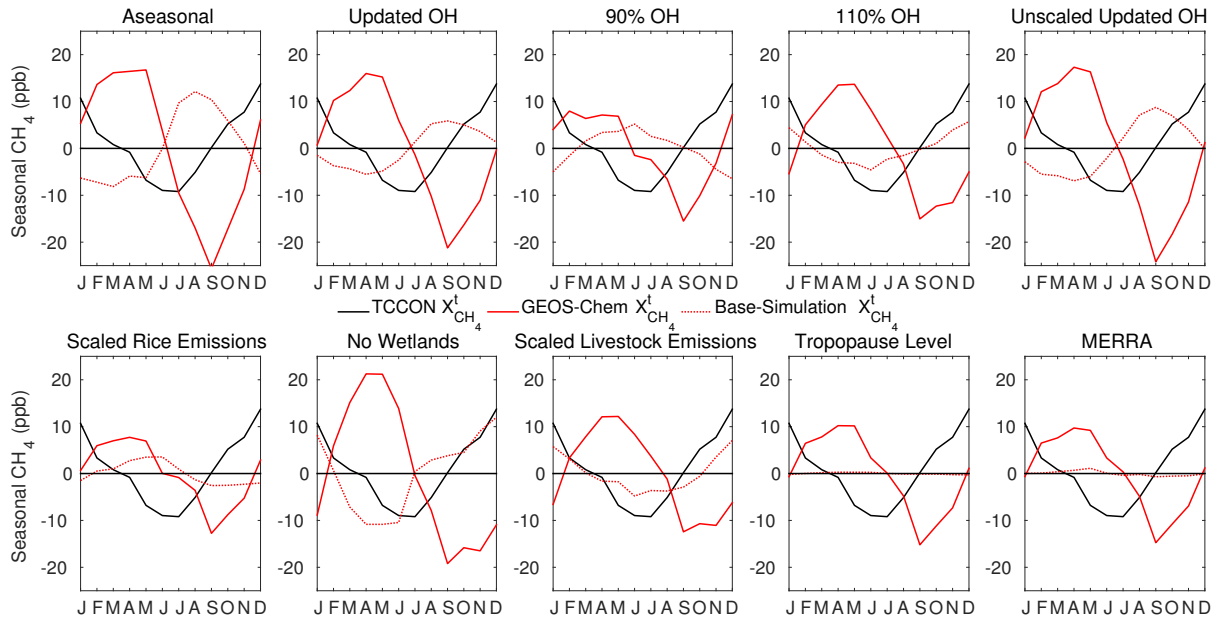
Figure 15. Seasonality of tropospheric methane ( X_{\text{CH}_4}^t ) at Park Falls for TCCON (black solid line), GEOS-Chem (red solid line), and the difference from the base simulation (dotted red line) for each of the sensitivity experiments, in ppb.
