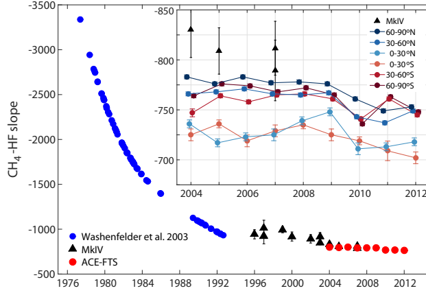
Figure 11. Long-term \text{CH}_4 -HF slopes from Washenfelder et al. (2003), MkIV, and updated ACE-FTS measurements. Inset: Time series of zonal pressure-weighted ACE-FTS slopes ( \beta ) used to calculate \hat{X}_{\text{CH}_4}^t , with error bars denoting the 2\sigma standard error. Zonal slopes are offset each year for visual clarity.
