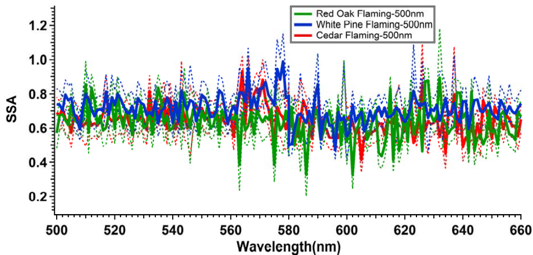
Figure 7. SSA of 500 nm particles from white pine, red oak, and cedar sampled during the flaming stage.
