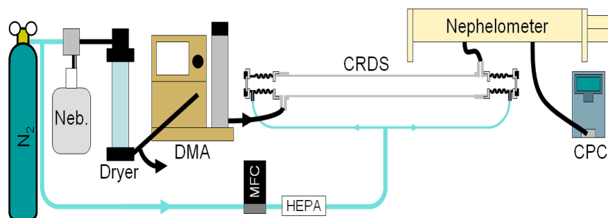
Figure 2. The integrated aerosol optical property measurement system
