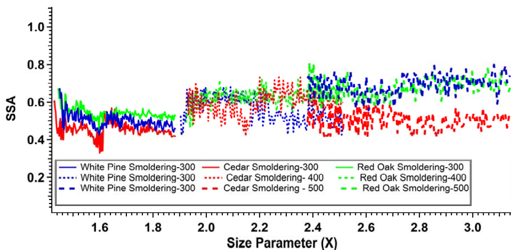
Figure 11. SSA as a function of size parameter for all samples in smoldering stage.
