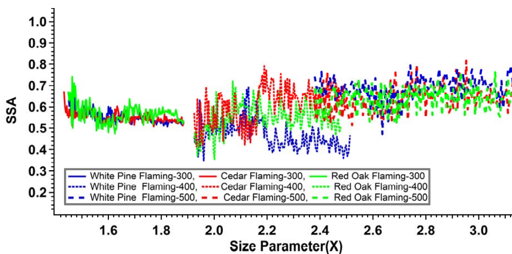
Figure 12 SSA as a function of size parameter for all samples flaming stage.
