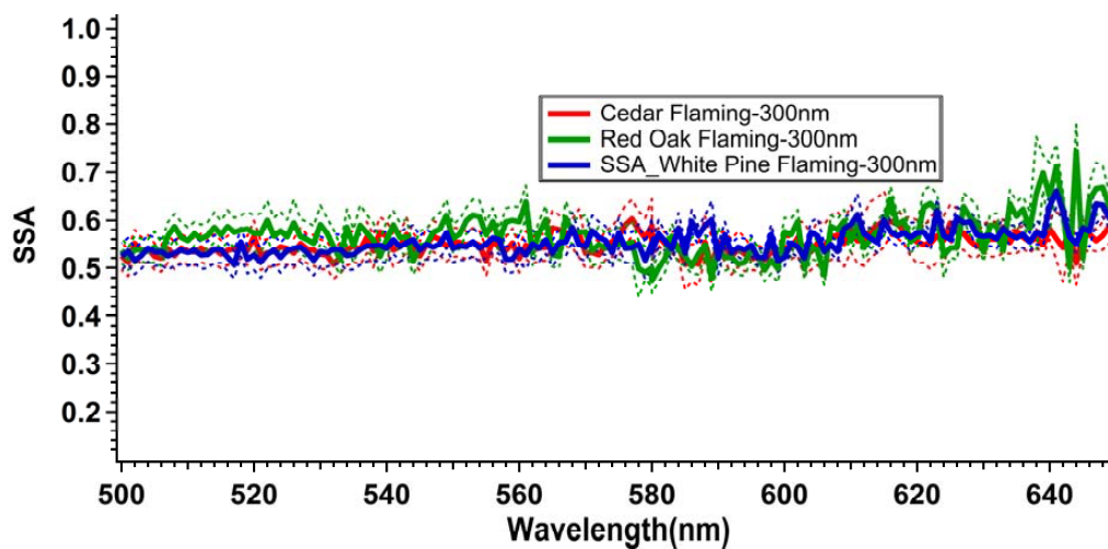
Figure 5. SSA of 300 nm particles from white pine, red oak, and cedar sampled during the flaming stage
