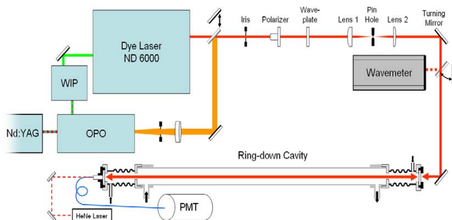
Figure 1. The laser and optical components of the CRDS instrument
