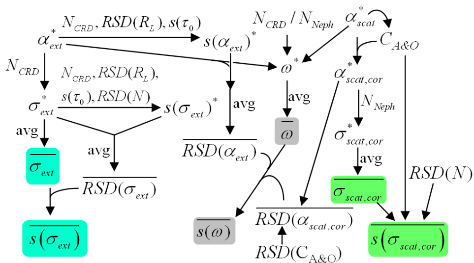
Figure 4. The calculation flow for determining average \sigma_{ext} , \sigma_{scat} , \omega , and their errors.
