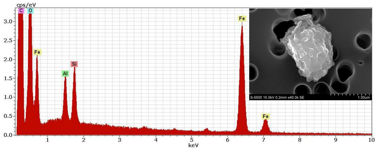
5 Figure 20: SEM based EDS spectrum and SEI of a particle from re-suspended sample S1009 from Mali. The composite particle contains iron (Fe) as the mineral goethite ( \text{FeO}(\text{OH}) ) and/or hematite ( \text{Fe}_2\text{O}_3 ) together with silicon (Si) and aluminum (Al) in the clay mineral kaolinite.
