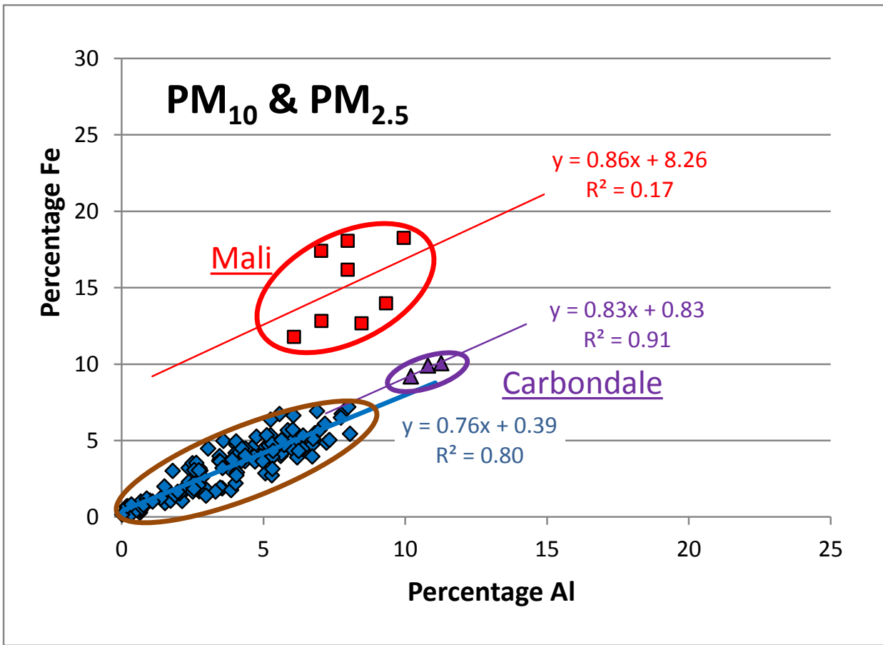
5 Figure 17: Plot showing the linear relationship between iron (Fe) and aluminum (Al) for 130 chemically analyzed soil re-suspensions. Three sample clusters can be identified with most (122) falling in one field (brown oval) with an average Fe/Al slope of 0.76. Samples from Mali (red oval) and Carbondale (violet oval) have slightly higher slopes. The high correlation and tight cluster of the largest (122 samples) group implies that the iron (Fe) is in part contained in the clay mineral structure or dispersed as colloidal oxihydroxide in the clay-like amorphous matrix.
