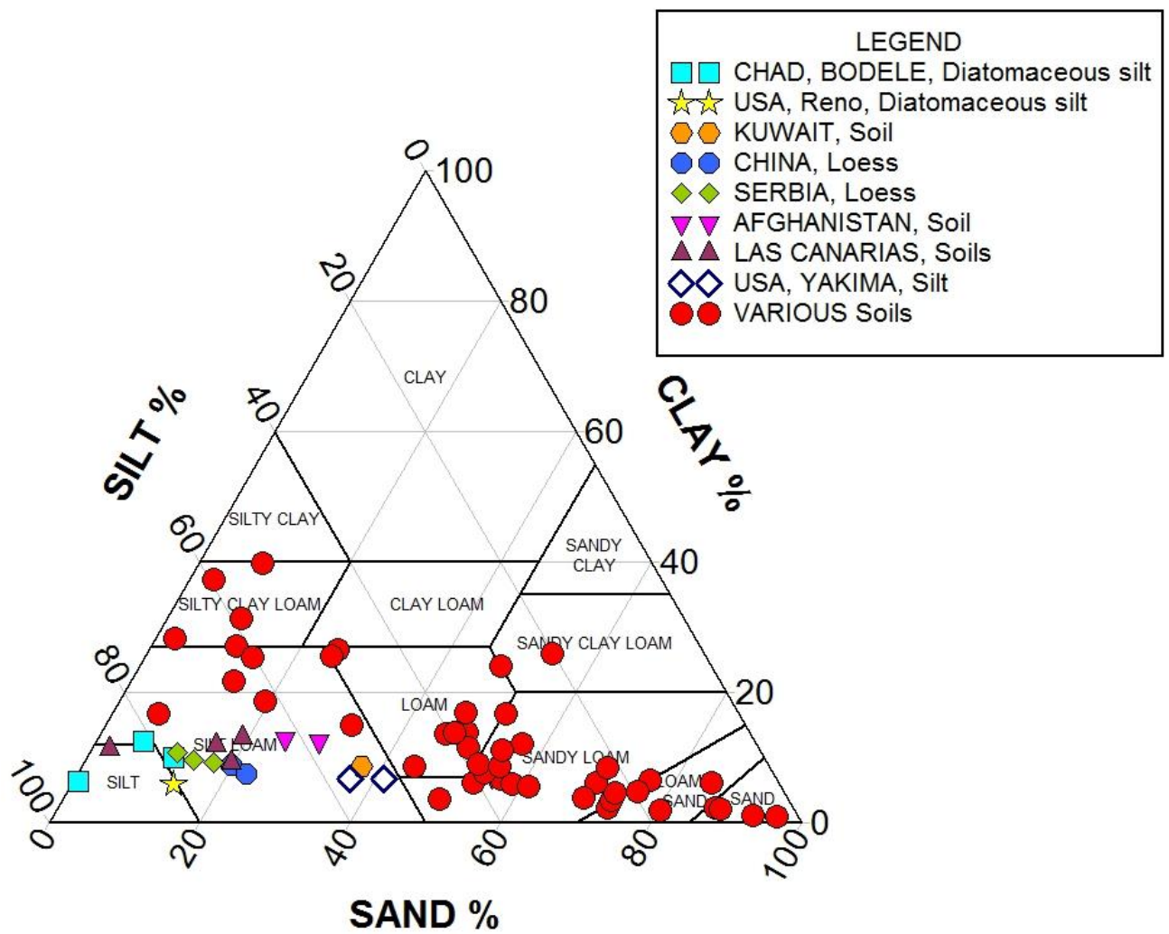
5 Figure 15: Size-class fractions grouped as clay (< 2 \mu\text{m} ), silt (2 - 62.5 \mu\text{m} ) and sand (62.5 – 600 \mu\text{m} ). Samples from regions with the greatest potential to be sources of airborne dust lie in the “silt loam” and “silt” fields with less than about 10% clay, including samples from known dust regions in Chad , China, Afghanistan, Kuwait, northwestern Africa, southeastern Europe and parts of western U.S.A.
