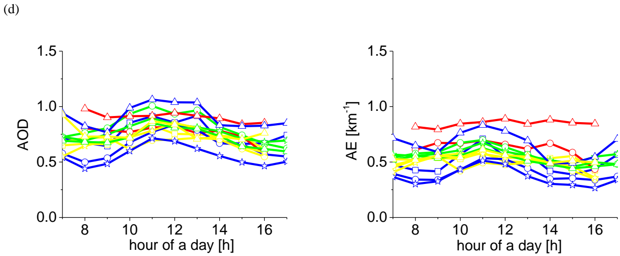
5 Figure 14: Seasonally averaged diurnal variations of TG x VCDs and AOD (left) and near surface values (right) of NO 2 (a), SO 2 (b), HCHO (c) and aerosols (d) from 2011 to 2014.
