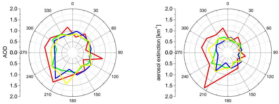
5 Figure 15: Dependencies of VCDs and AODs (left) and near-surface VMRs and AEs (right) of \text{NO}_2 (a), \text{SO}_2 (b), HCHO (c) and aerosols (d) on wind directions for individual seasons (different colours).
