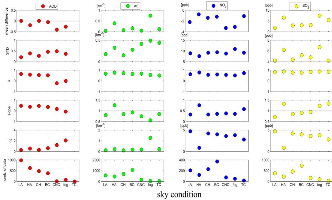
5 Figure 9: Mean absolute differences, standard deviations as well as correlation coefficients (R), slopes and intercepts derived from linear regressions of the AODs, near-surface AEs, NO 2 and SO 2 VMRs between MAX-DOAS and independent techniques for different seasons for different sky conditions. The corresponding numbers of data are shown in the bottom panel. Different colours denote AOD (compared with the Taihu AERONET level 1.5 data sets), AE (compared with the nearby visibility meter) and NO 2 and SO 2 (compared with the nearby long path DOAS instrument).
