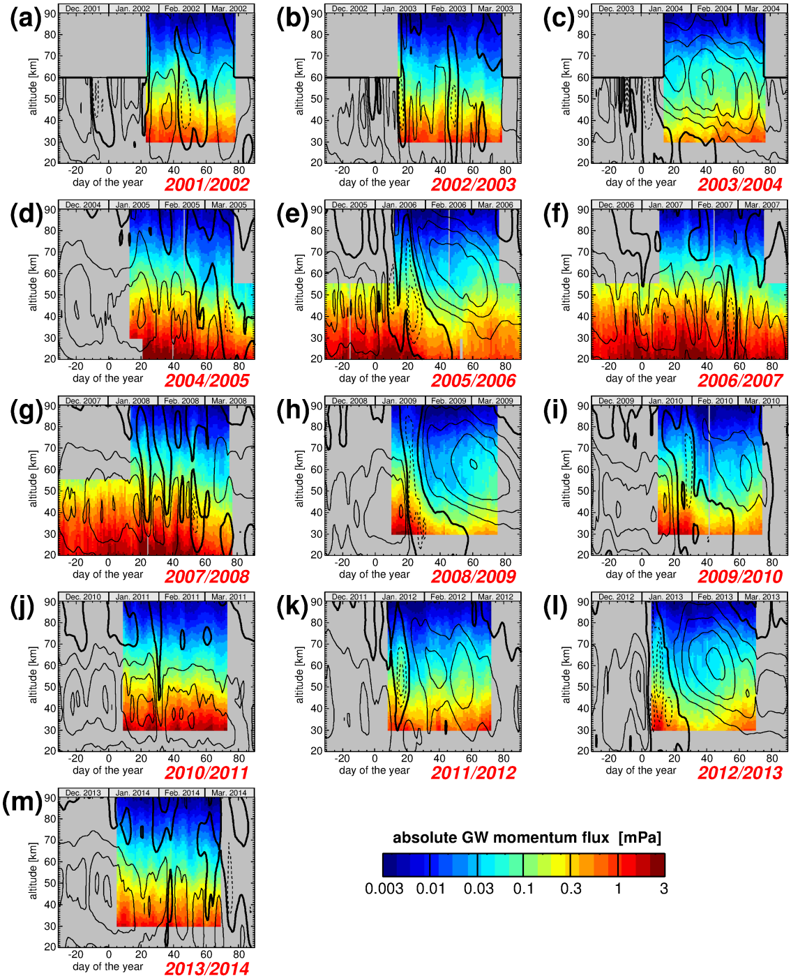
Figure 5. Same as in Fig. 3, but for gravity wave absolute momentum fluxes at 60° N–80° N. Momentum fluxes are given in mPa on a logarithmic color scale. Like in Fig. 1, overplotted contour lines indicate zonal average zonal winds at 60° N–80° N in steps of 20 m s -1 .
