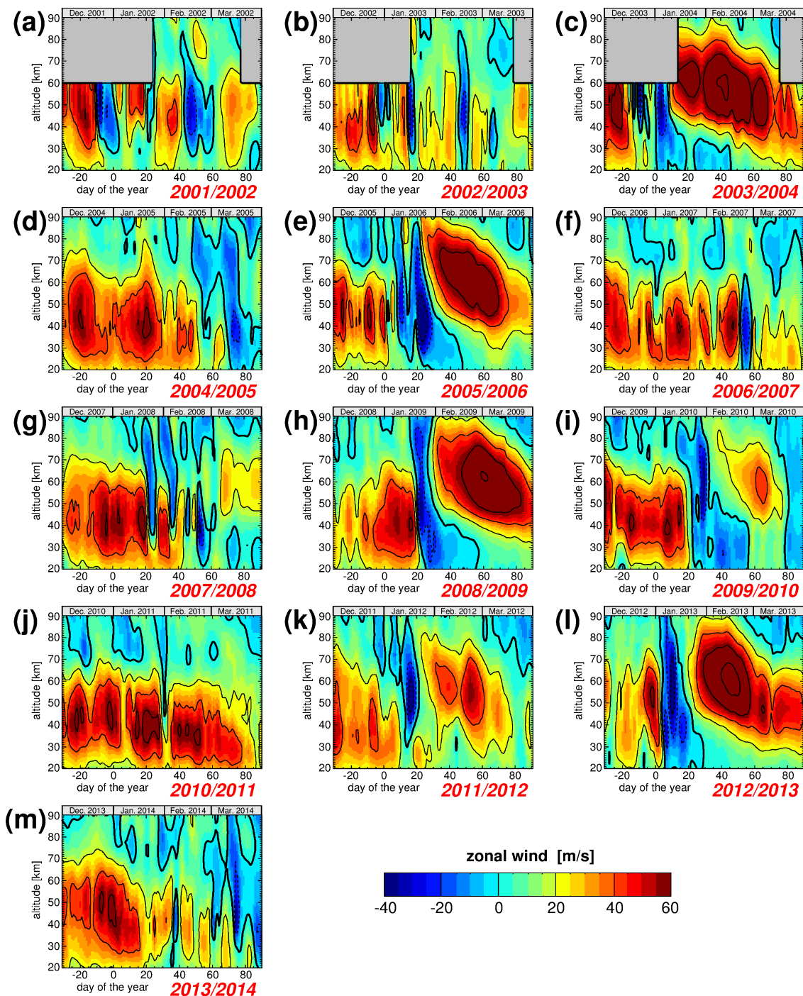
Figure 1. Altitude-time cross-sections of daily 60^{\circ}\text{N} – 80^{\circ}\text{N} zonal average zonal wind in \text{m s}^{-1} from ERA-Interim, MLS Aura and SABER combined. The time scale on the x-axis is given in "days of the year" (doy) with 1 January 00:00 UT as doy=0. Overplotted contour lines have a contour increment of 20 \text{ m s}^{-1} . Westward (eastward) winds are indicated by dashed (solid) contour lines. The zero wind line is bold solid. Times and altitudes where no data are available are marked in gray.
