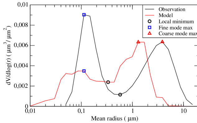
Figure 10. Method for the local minima and maxima values estimation. This example corresponds to the ASD for Athens, 23 July 2013, 14:00 UTC.
