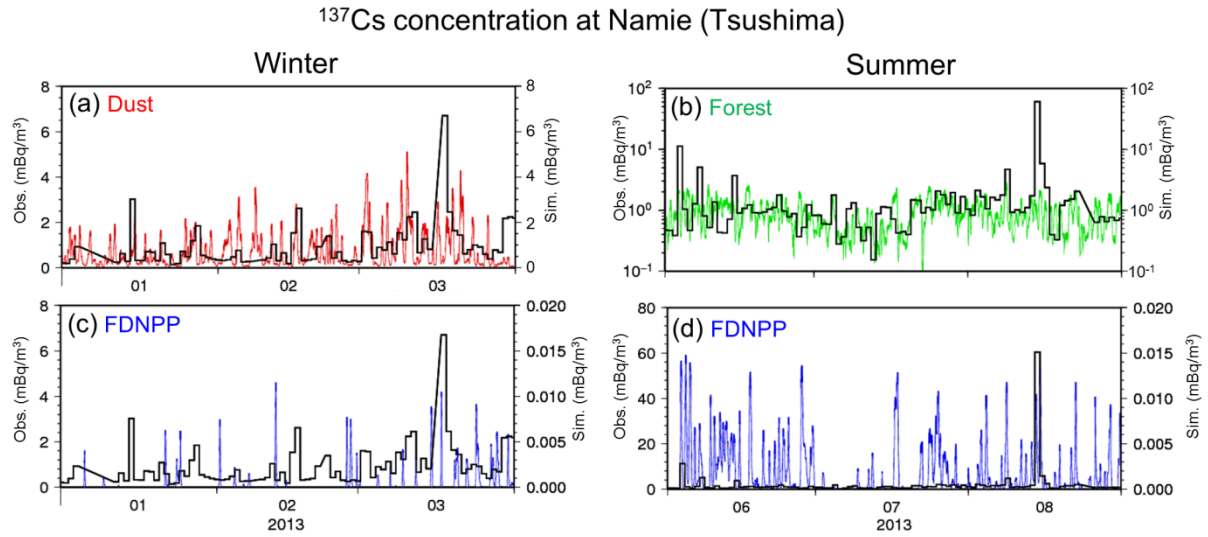
Figure 9. Time series of observed (black) and simulated (colors) ^{137}\text{Cs} surface air concentration at Namie (a, c) in winter from January to March and (b, d) in summer from June to August, 2013. The colors of the lines are the same as in Fig. 7 but the time variation is hourly. The shaded areas indicate the range of ^{137}\text{Cs} concentrations obtained when the simulations were run using the optimized parameter ranges E_c = 0.03 - 0.05 and v_d = 0.05 - 0.1 cm/s.
