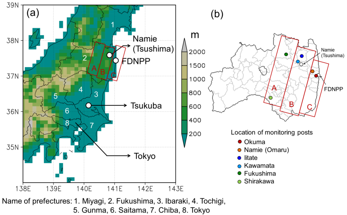
Figure 1. (a) The model domain showing the model terrestrial elevation, observation sites, and other locations described in the study. The linear distances from FDNPP to Namie (Tsushima district, Namie town), Tsukuba and Tokyo are approximately 30 km, 170 km, and 220 km, respectively. The numbers denote prefectures: 1. Miyagi, 2. Fukushima, 3. Ibaraki, 4. Tochigi, 5. Gunma, 6. Saitama, 7. Chiba, and 8. Tokyo. (b) Fukushima prefecture and (colored circles) the locations (village, town, or city name) of monitoring posts used in this study (see Fig. C1). The letters in both (a) and (b) denote the name of the area based on geographical features: A. Nakadori valley, B. Abukuma highland, and C. Hamadori coastal area.
