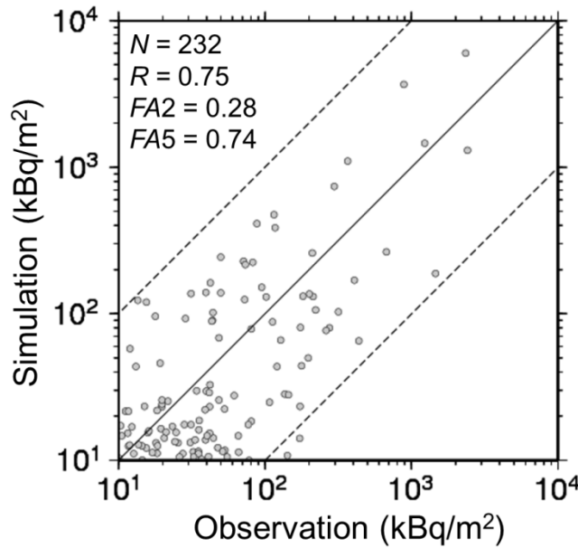
Figure 5. Scatterplot between the observational data and the simulation results for ^{137}\text{Cs} deposition ( \text{kBq/m}^2 ). The deposition parameters of the simulation in the figure are E_c = 0.04 and v_d = 0.1 \text{ cm/s} . N indicates the number of samples, and the statistical measures R , FA2 , and FA5 are described in Table 2.
