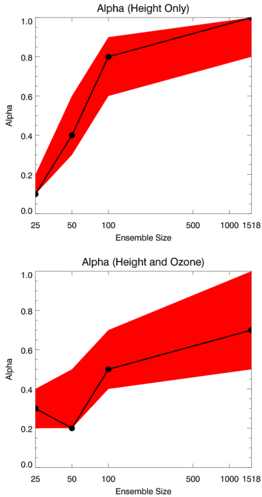
Fig. 5. Black circles indicate optimal blending coefficient, \alpha (unitless), as a function of ensemble size for Z assimilation (top) and Z/O_3 assimilation (bottom). The range values in red indicate hybrid experiments with WEP values within 0.5% of the maximum WEP for each ensemble size.
