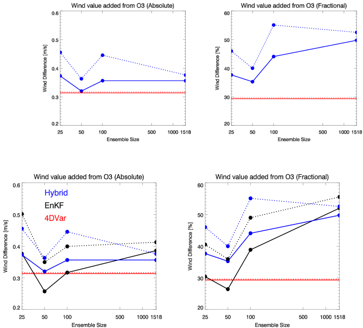
Fig. 8. Differences in the global RMSE of the vector wind between experiments that assimilate Z only and experiments that assimilate both Z and O_3 . For each ensemble size, the final RMSE of the vector wind is calculated for each experiment and then the differences are taken. Left: the absolute difference in \text{ms}^{-1} . Right: the fractional difference (i.e., the difference from (a) divided by the RMSE of the vector wind for Z only) in %. Red is 4DVar, blue is hybrid, and black is EnKF. Solid circles indicate the values for each ensemble, while solid (dotted) connecting lines differentiate results without (with) NMI post-processing. Note that larger positive numbers indicate smaller errors due to adding O_3 .
