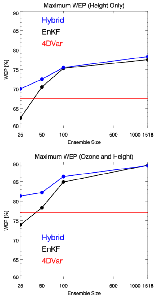
Fig. 7. Solid circles with connecting lines indicate maximum WEP (in %) as function of ensemble size for Z assimilation (top) and Z/O_3 (bottom) assimilation. WEP is shown for EnKF (black), and hybrid (blue). Red lines indicate the maximum WEP for 4DVar.
