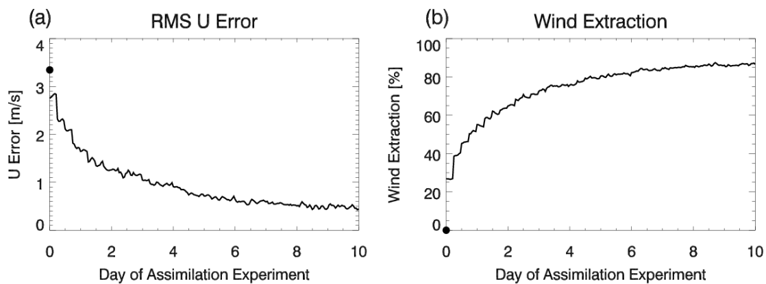
Fig. 2. (a) Global RMSE of the zonal wind (in \text{ms}^{-1} ), and (b) Wind Extraction Potential (in %) for the optimal 100 member hybrid 4DVar for Z/O 3 assimilation. Black circles indicate the values at the start of the assimilation experiment.
