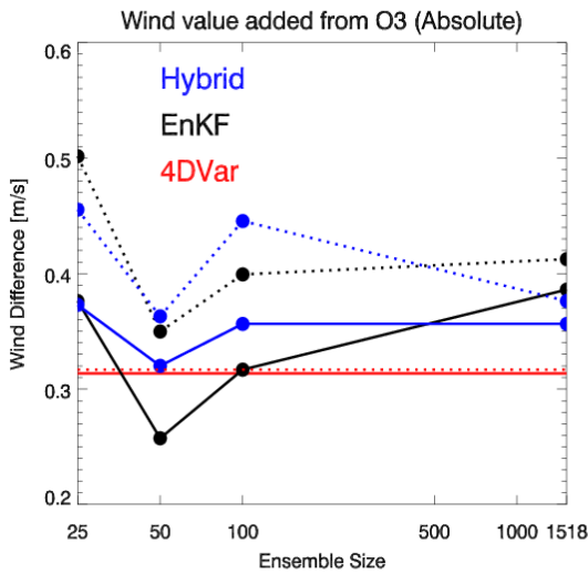
Fig. 78. Global RMS vector wind error differences between experiments that assimilate Z assimilation only and experiments that assimilate both and Z and O 3 assimilation . For each ensemble size, the final vector wind errors are calculated for each experiment and then the differences are taken. Left: absolute difference in ms -1 . Right: fractional difference (i.e., the difference divided by the vector wind error for Z only assimilation) in %. Red is 4DVar, and blue is hybrid, and black is EnKF. Solid (dotted) lines indicate results without (with) NMI post-processing. Note that larger positive numbers indicate smaller errors due to adding O 3 .
