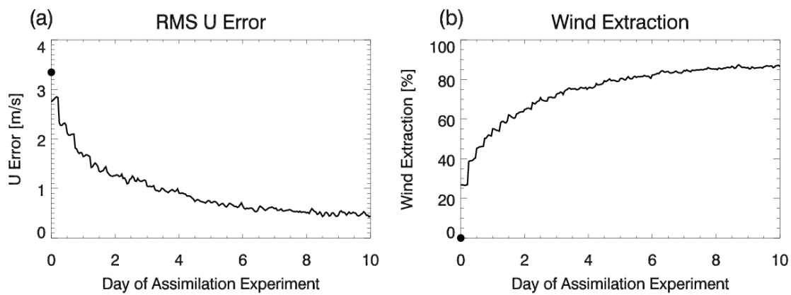
Fig. 2. (a) Global RMSE of the zonal wind (in \text{ms}^{-1} ), and (b) Wind Extraction Potential (in %) for the optimal 100 member hybrid 4DVar assimilation of Z and O 3 . Black circles indicate the values at the start of the assimilation experiment.
