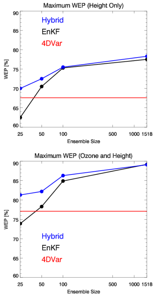
Fig. 67. Maximum WEP (in %) as function of ensemble size for Z assimilation (top) and Z/O 3 (bottom) assimilation. WEP is shown for 4DVar (red), EnKF (black), and hybrid (blue).
