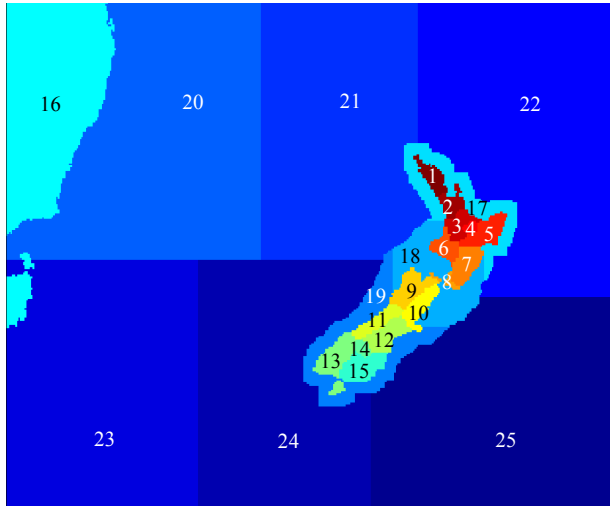
Figure 8. Regional partitioning and indices in the inversion.
