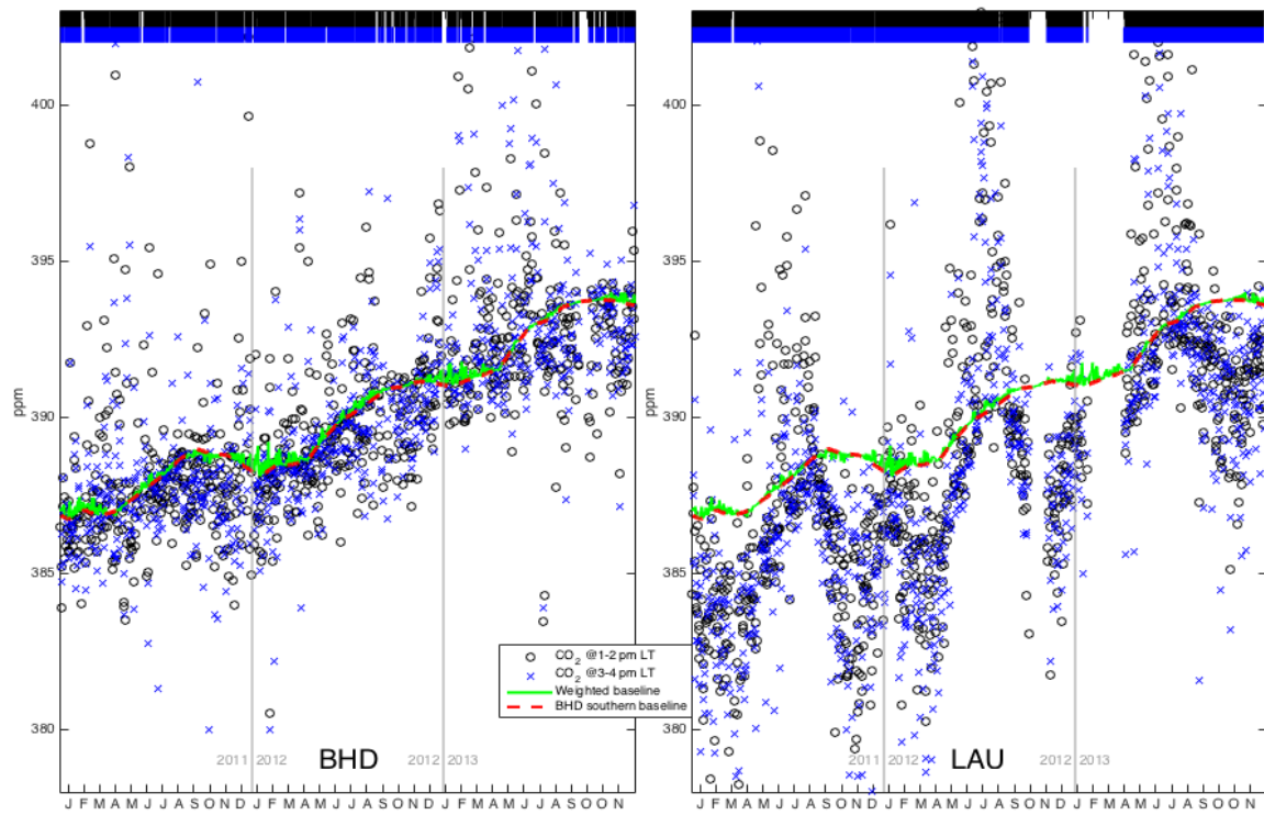
Figure 1. \text{CO}_2 observations from BHD and LAU, twice-daily at 13:00-14:00 and 15:00-16:00 LT, through 2011-13. The BHD southern baseline is shown along with the weighted baseline used in the inversion. Gaps in the coloured bars at the top indicate days when no observations are available.
