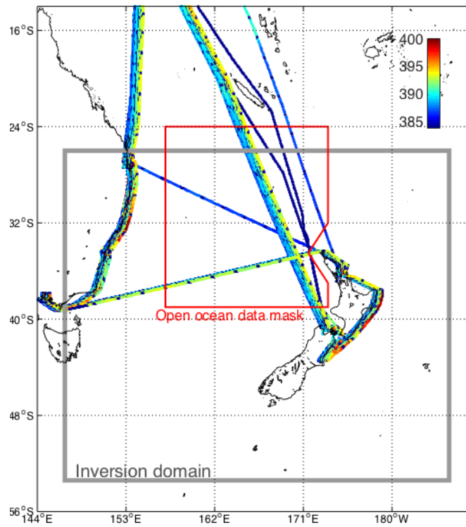
Figure 3. Voyages of the Ship of Opportunity "Trans Future 5". Ship tracks have been slightly spread longitudinally to allow one to differentiate individual cruises (more recent cruises are to the right). Colors give the in situ CO 2 concentration. Measurements made inside the open ocean mask were used in the northern baseline analysis. The inversion domain is outlined in gray.
