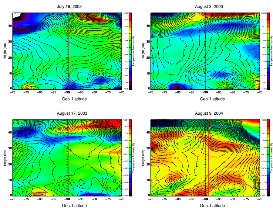
Figure 8. 24-hr time differenced contour plots of geopotential height (black contours) and temperatures obtained from ECMWF Reanalysis from 0-50 km along the direction of the ray path for waves observed on July 19, 2003 (top left), August 3, 2003 (top right), August 17, 2003 (bottom left) and August 9, 2004 (bottom right), as determined by our GROGRAT model runs. Ticks on contour lines point to lower geopotential height. Vertical red line marks the latitude at which the ray terminates, and the corresponding red 'X' denotes the location of the wave source.
