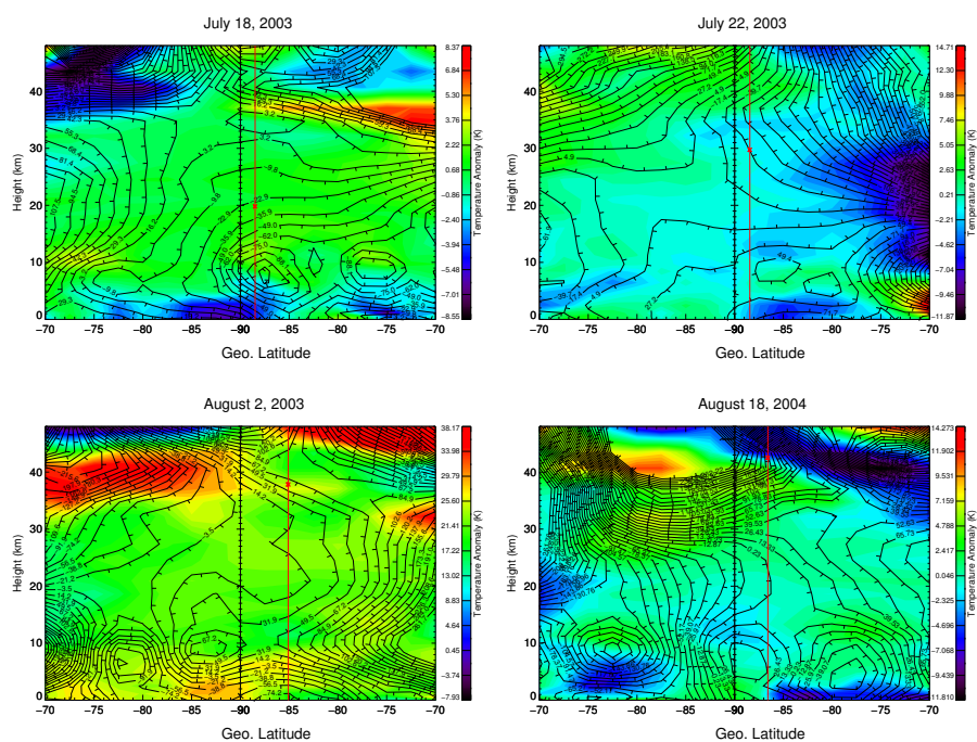
Figure 7. 24-hr time differenced contour plots of geopotential height (black contours) and temperatures obtained from ECMWF Reanalysis from 0-50 km along the direction of the ray path for waves observed on July 18, 2003 (top left), July 22, 2003 (top right), August 2, 2003 (bottom left) and August 18, 2004 (bottom right), as determined by our GROGRAT model runs. Ticks on contour lines point to lower geopotential height. Vertical red lines mark the latitude at which the rays terminate, and the corresponding red 'X' denotes the location of the wave source.
