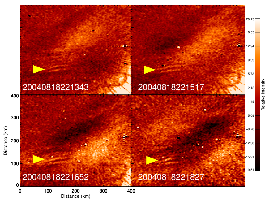
Figure 2. Processed Na image from August 18, 2004. The images were unwarped onto a 400 x 400 km geographic grid (shown in the bottom left image) with the positive y-axis corresponding to 0^\circ longitude. Yellow arrows mark the location of the observed wave in each image. Time stamps are shown in the bottom left of each image, and is read as YYYYMMDDHHMMSS. The sequence of images starts at the top left, and follows to the top right, bottom left, and finally bottom right.
