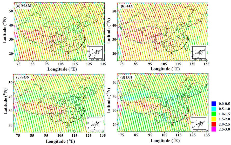
Figure 4. Spatial distributions of climatological PBLHs derived from CALIOP at 1330 BJT in (a) spring (March-April-May, MAM), (b) summer (June-July-August, JJA), (c) autumn (September- 5 October-November, SON) and (d) winter (December-January-February, DJF) during the period 2011 - 2014. Horizontal resolution is resampled to 20 km along the ground track.
