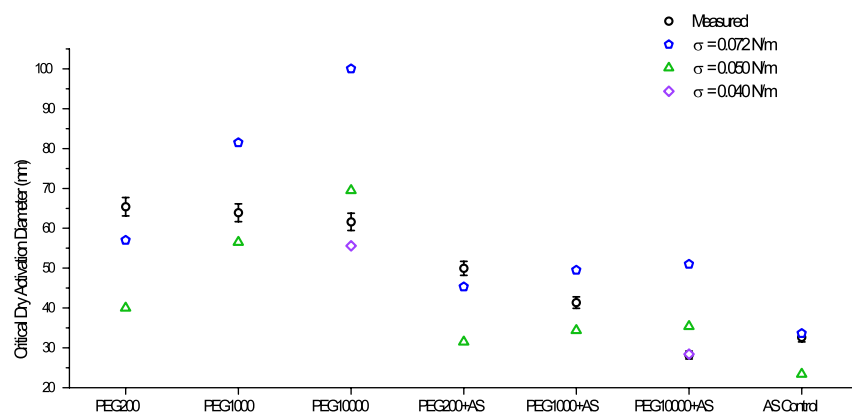
Update Figure 3. Critical dry particle diameters ( D_{crit} ) at a water supersaturation of 0.8% at 298K for the PEG, PEG-AS and, AS Control aerosol systems determined from CCN measurements (black circles) and calculated using AIOMFAC with classical Köhler theory assuming a range of droplet surface tensions ( \sigma ). Values of D_{crit} were determined from CCN measurements by fitting the activation-fraction measurements with sigmoidal curves, as shown in Figure 2, and determining the dry particle diameter associated with an activation fraction of 50% using these curves. Error bars on D_{crit} indicate an assumed uncertainty in DMA-transmitted particle diameter of 3.5%.
