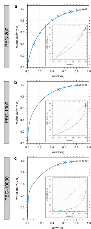
Figure A2. Comparison of measured and predicted water activity vs. mixture composition at 298.15 K. Experimental data (crosses) are from Ninni et al. (1999). The blue curves show the specific AIOMFAC predictions for the mole fraction based water activity of aqueous PEG200 (a), PEG1000 (b) and PEG10,000 (c) mixtures vs. mass fraction of water, w(\text{water}) . The insets show water activity vs. mole fraction of water, x(\text{water}) ; the dotted diagonal line shows the water activity of a hypothetical ideal solution. The deviations between ideal and non-ideal a_w curves indicate the pronounced deviation from ideal solution behavior with increasing molar mass (i.e. increasing molecular size) of the PEG component (from a to c).
