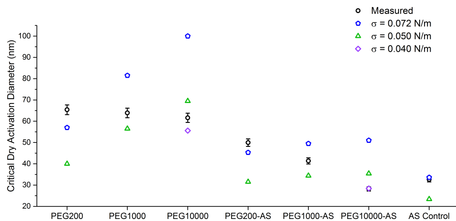
Figure 3. Critical dry particle diameters ( D_{crit} ) at a water supersaturation of 0.8% at 298K for the PEG, PEG-AS and, AS Control aerosol systems determined from CCN measurements (black circles) and calculated using AIOMFAC with classical Köhler theory assuming a range of droplet surface tensions ( \sigma ). Values of D_{crit} were determined from CCN measurements by fitting the activation-fraction measurements with sigmoidal curves, as shown in Figure 2, and determining the dry particle diameter associated with an activation fraction of 50% using these curves. Error bars on D_{crit} indicate an assumed uncertainty in DMA-transmitted particle diameter of 3.5%.
