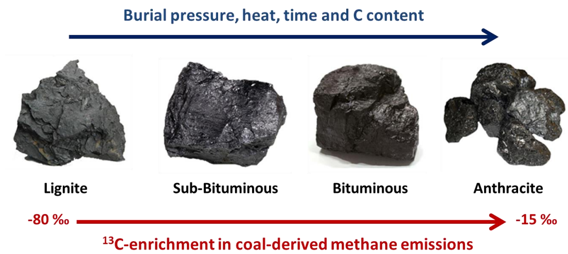
Figure 1 Coal maturation process.
