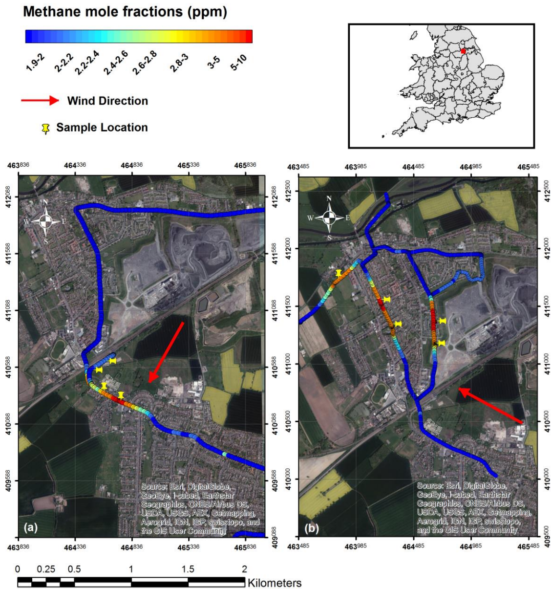
Figure 3 ArcGIS maps of methane mole fractions recorded downwind of Hatfield Colliery on July (a) and September 2013 (b). Grid Coordinates are displayed in the National British Coordinate System.
