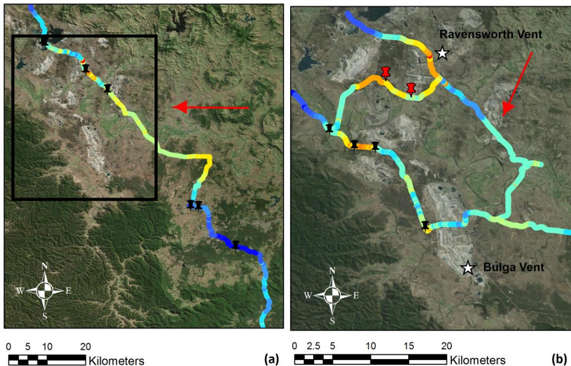
Figure 2 Methane mole fractions recorded in the Hunter Coalfield on 12th March 2014 (a) and during a more detailed survey of the area highlighted by the black square on 18th March 2014 (b). Source: Esri, DigitalGlobe, GeoEye, i-cubed, Earthstar Geographics, CNES/Airbus DS, USDA, USGS, AEX, Getmapping, Aerogrid, IGN, IGP, swisstopo and the GIS User Community.
