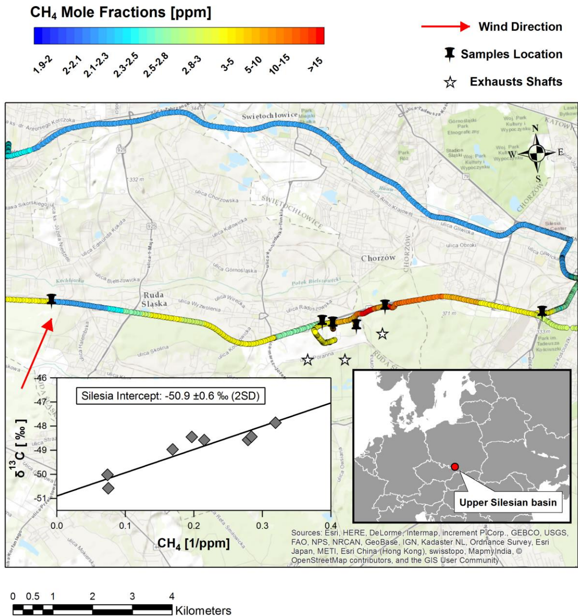
Figure 5 ArcGIS map of methane mole fractions recorded in the Upper Silesian basin in June 2013. White stars represent the KWK Wujek deep mine exhausts shafts. The embedded graph is the Keeling Plot based on samples collected downwind the KWK Wujek deep mine in June 2013. Errors on the y-axis are within 0.05 ‰ and on the x-axis 0.0001 ppm -1 , and are not noticeable on the graph.
