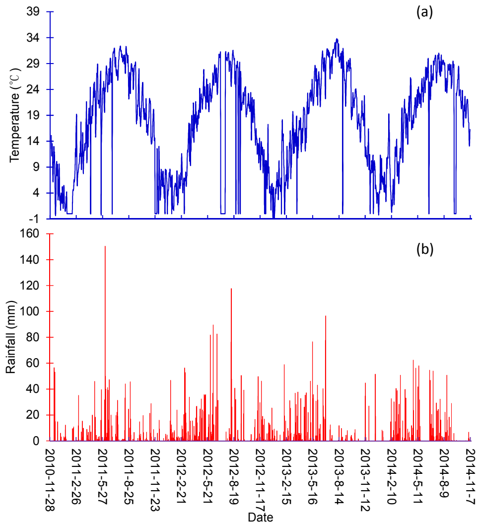
Fig. 1 The daily air temperature (a) and rainfall (b) throughout the whole observational period
