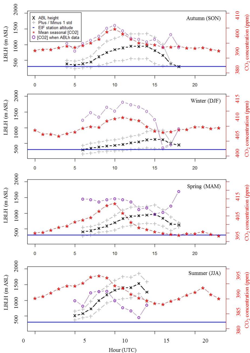
Figure 7. Diurnal cycles of the hourly LBLH estimate means ( \pm 1\sigma ) and of \text{CO}_2 hourly means observed by season at QUALAIR and EIF, respectively. Time is in hour UTC. The horizontal line is the elevation of EIF. The violet circles give the \text{CO}_2 concentration (according to the red scale) at the moments when the LBLH was measured as well.
