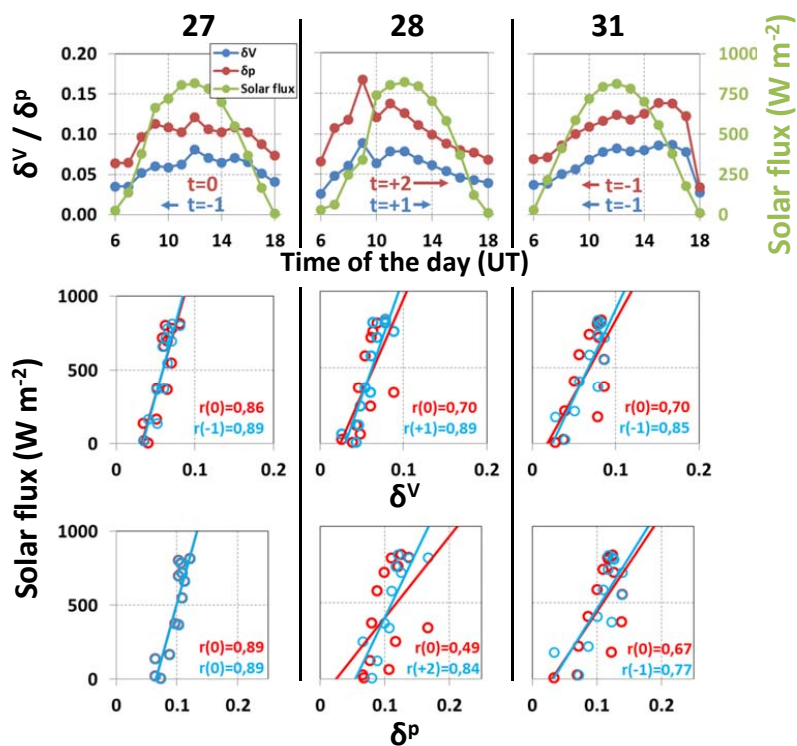
Figure 8. (top) Diurnal evolution of \overline{\delta^V} , \overline{\delta^P} and solar fluxes on 27, 28 and 31 March between 06 and 18 UT; (center) scatter plot of the solar flux vs. \overline{\delta^V} ; (bottom) scatter plot of the solar flux vs. \overline{\delta^P} . In each scatter plot, straight lines are linear regression lines; the red color corresponds to t=0 ; the blue color corresponds to t=t_{opt} . The values of r(t) are reported in each scatter plot.
