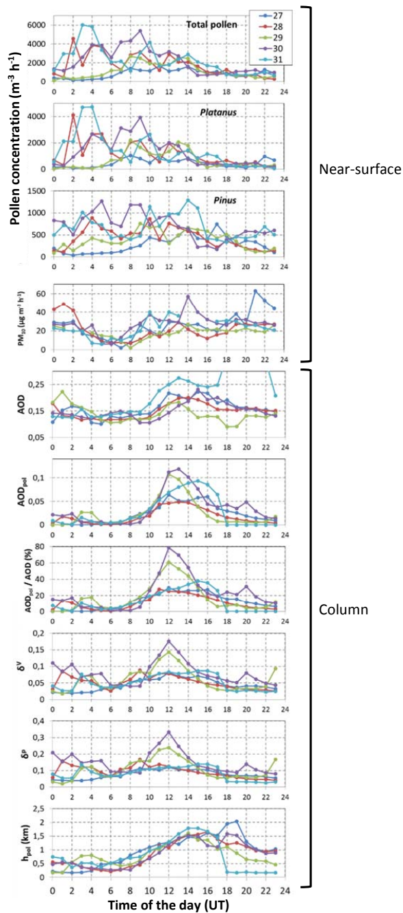
Figure 5. Daily cycle for all five days of the pollination event of the total pollen, the Platanus and the Pinus concentration, PM_{10} , AOD, AOD_{pol} , AOD_{pol}/AOD , \delta^v , \delta^p and h_{pol} (see legend in the top plot).
