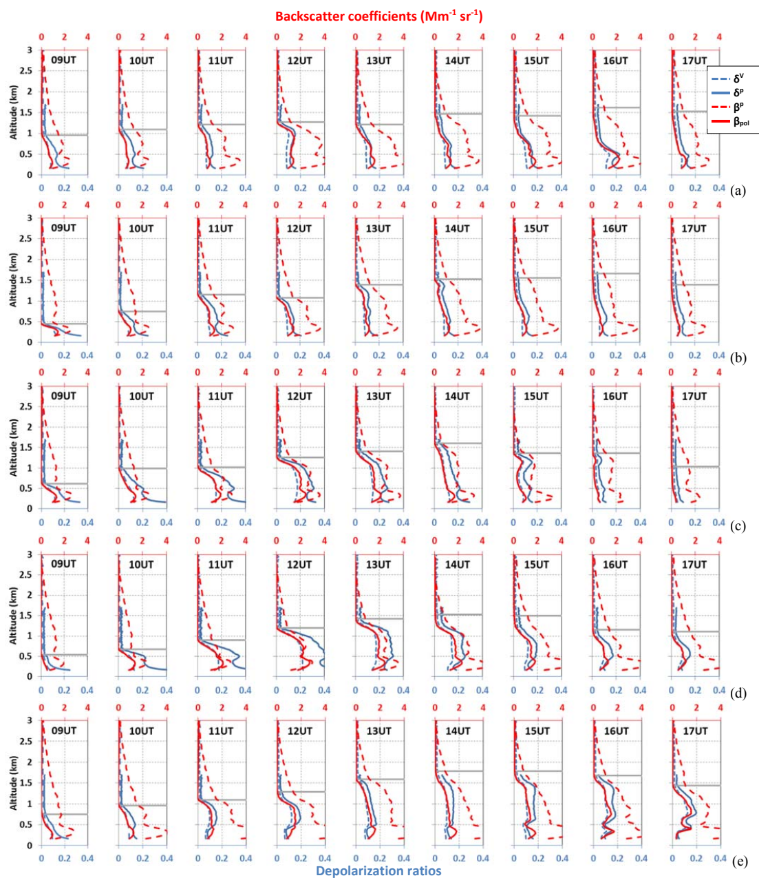
Figure 4. Diurnal time series of the hourly vertical distribution of the particle backscatter coefficient ( \beta^p ), the pollen backscatter coefficient ( \beta_{pol} ), the volume depolarization ratio ( \delta^v ) and the particle depolarization ratio ( \delta^p ) on (a) 27, (b) 28, (c) 29, (d) 30 and (e) 31 March, 2015.
