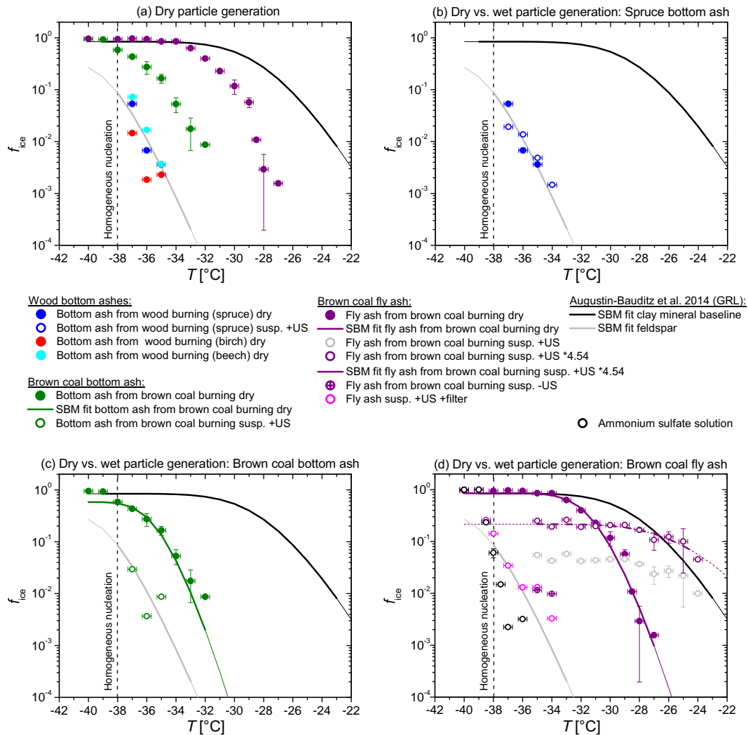
Figure 3. Ice fraction f_{ice} as a function of temperature T for ash particles from dry (full circles, (a)) and wet generation (open circles, (b), (c), (d)) with D_{p,el} = 300 nm. Error bars represent the LACIS temperature error of 0.3 K and the f_{ice} standard deviation of three or more measurements, respectively. A scaling factor of 4.54 was applied to the fly ash suspension measurements to account for the occurrence of crystals during wet particle generation. The solid and dashed lines represent the SBM fits to selected samples from this work and to data published in Augustin-Bauditz et al. (2014), all for D_{p,el} = 300 nm. Parameters for the SBM fits are given in Table 4. The feldspar sample from Augustin-Bauditz et al. (2014) is composed of 76 % microcline (K-feldspar) and 24 % albite (Na-feldspar). The clay mineral baseline corresponds to different kinds of mineral dust which featured a similar immersion freezing behavior after coating with sulfuric acid. The homogeneous region is determined by investigating the immersion freezing behavior of highly diluted ammonium sulfate droplets (black open circles, (d)).
