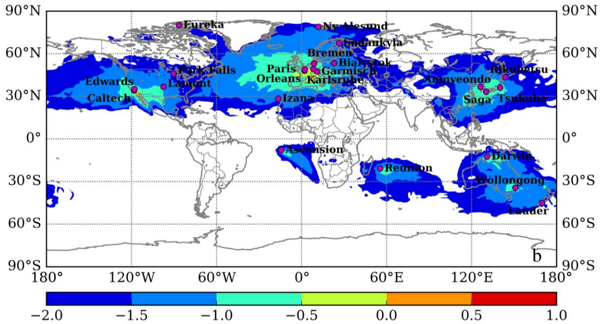
Fig. 1. Global distribution of the sensitivity of CO 2 concentrations ( \text{ppm} (\mu\text{mol} (\text{m}^2\text{s})^{-1})^{-1} ) with respect to the concentrations in adjacent cells, calculated using the FLEXPART model with a resolution of 1.0° for the 23 TCCON operational sites: a) tracer simulation initialized at the level of 1000 m, b) tracer simulation initialized at the level of 3000 m that corresponds to 700 hPa based on the International Standard Atmosphere for dry air.
