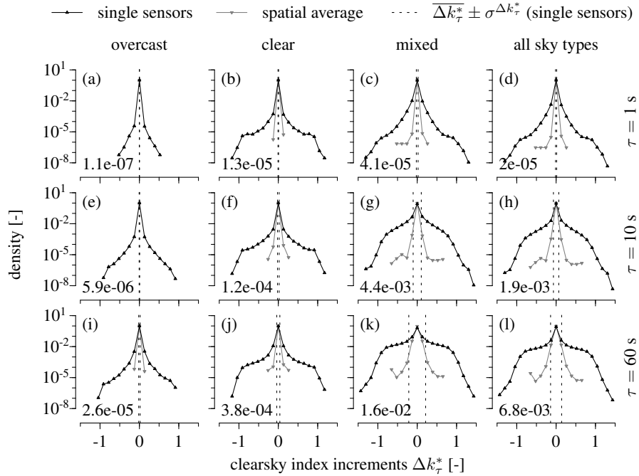
Figure 5. Statistics of clearsky index increments \Delta k^* for different time lags \tau , based on data from the Jülich campaign. The first three columns display distributions conditioned on different sky types, while the rightmost column presents the combined statistics for all sky types. The estimated probability density functions of all single sensors (solid black lines) are supplemented with the range of \pm one standard deviation \sigma^{\Delta k^*} around their means \overline{\Delta k^*} (dashed black lines), and contrasted to the much narrower distributions of the spatially smoothed average of all pyranometers (solid gray lines). The respective average probabilities P(\Delta k^* = \pm 0.5) of single sensors to fluctuate by \pm 0.5 are quoted in each panel.
